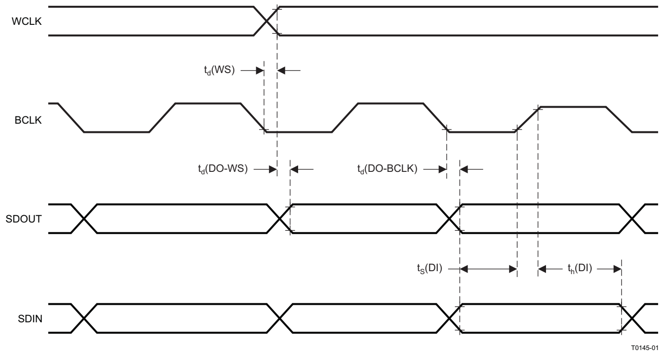
图 1. I²S, Left-Justified and Right-Justified Format Timing in Master Mode
