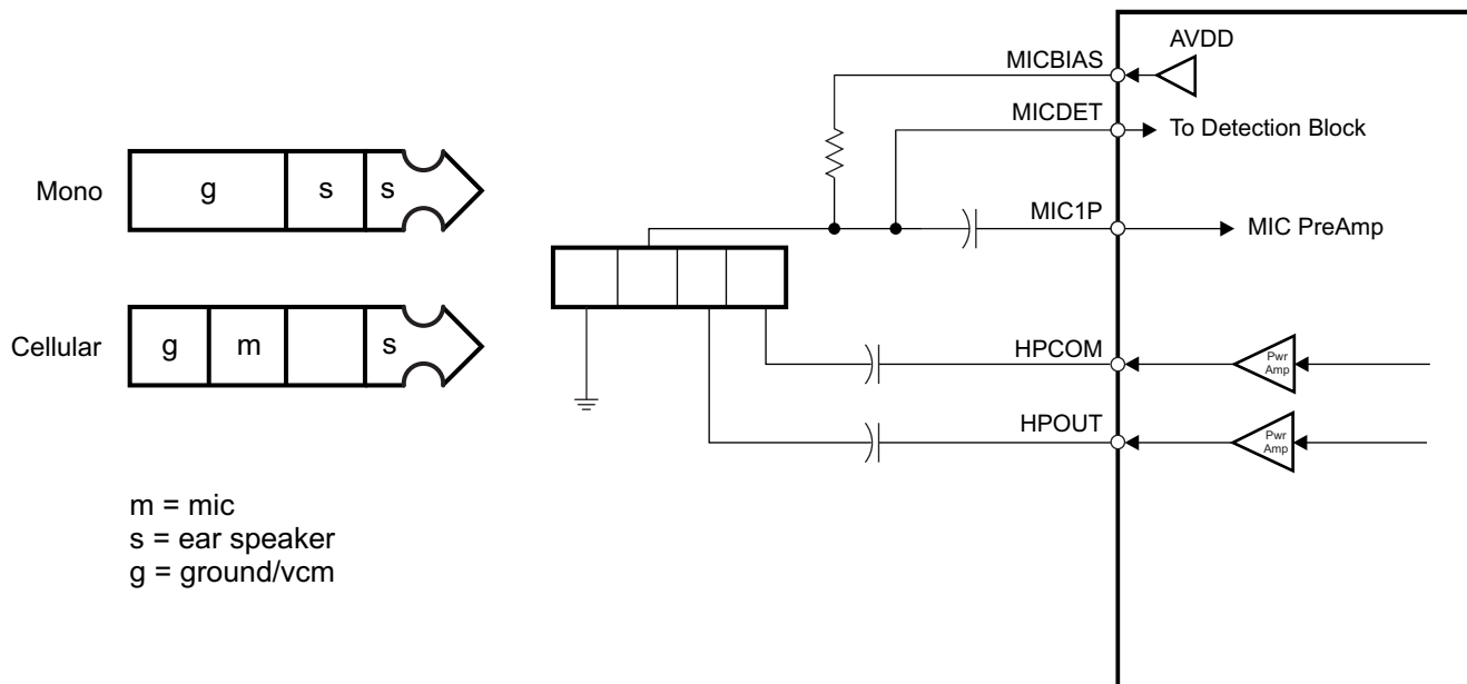
⊠ 25. Configuration of Device for Jack Detection Using an AC-Coupled Mono Headphone Output Connection
