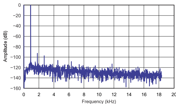
Figure 9-2. DAC to Line Output FFT at 1-kHz Signal Plot
