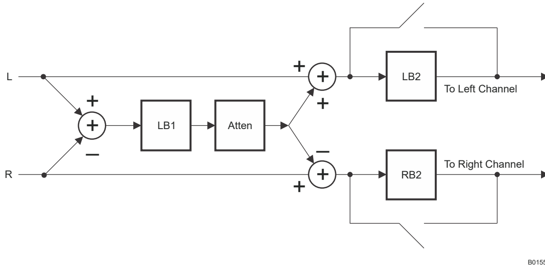
图 7-3. Architecture of Digital Audio Processing With 3-D Effects Enabled
