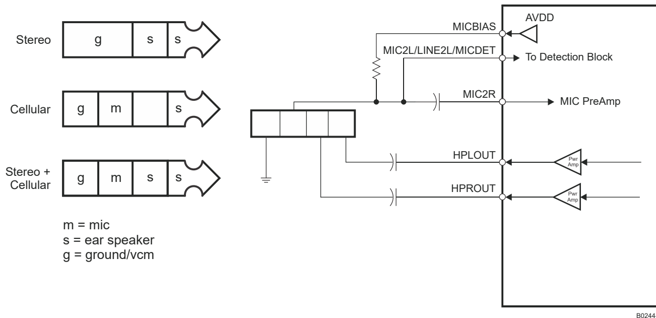
Figure 7-9. Configuration of Device for Jack Detection Using AC-Coupled Stereo Headphone Output Connection
