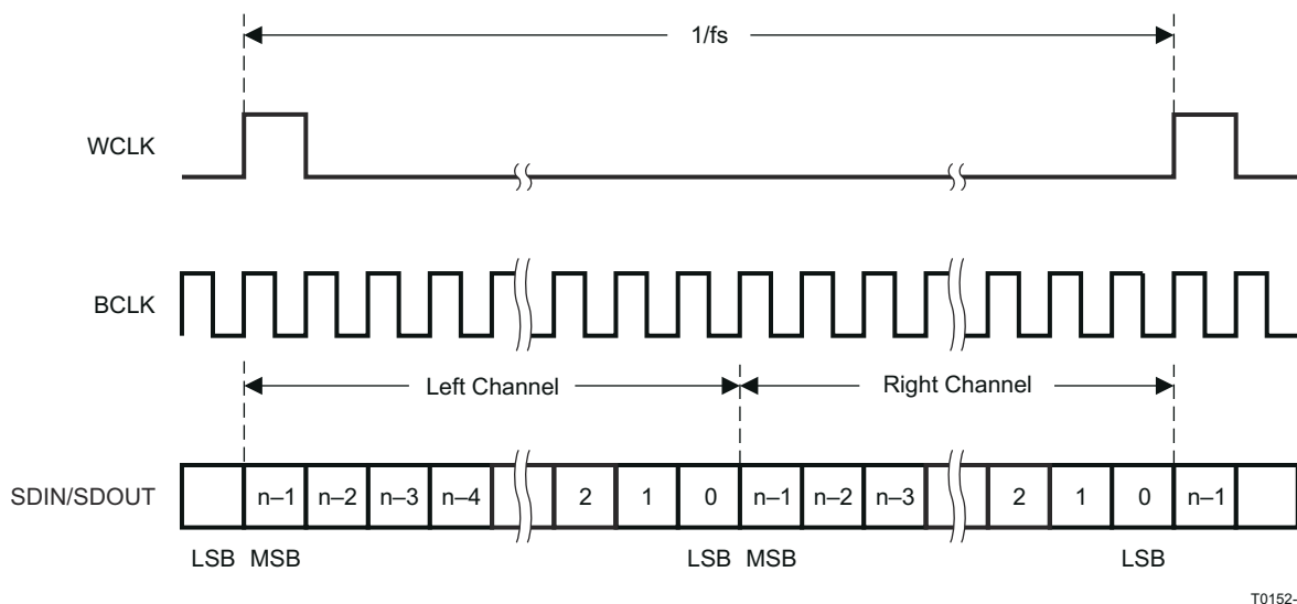
図 7-19. DSP Serial Data Bus Mode Operation
