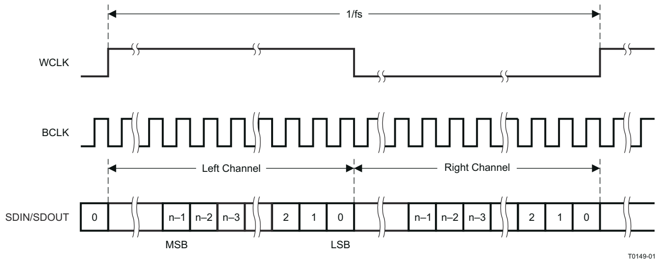
図 7-16. Right-Justified Serial Data Bus Mode Operation
