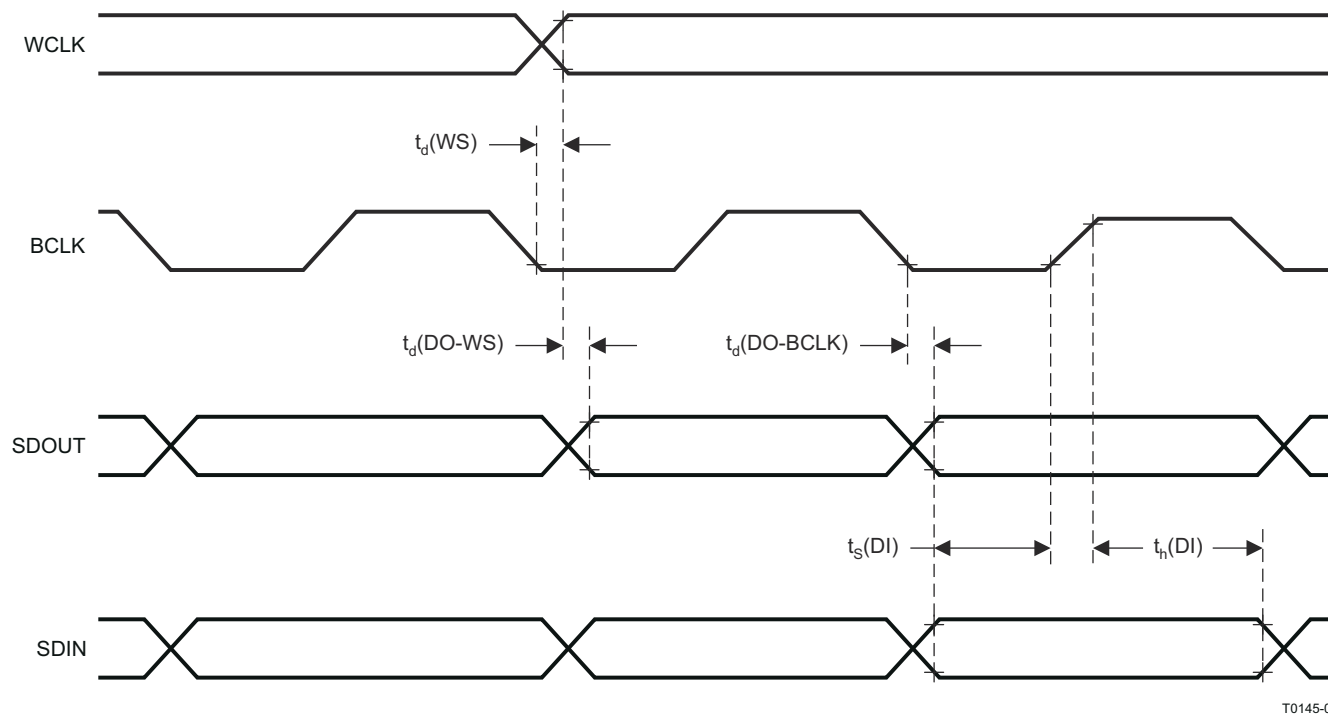
Figure 6-1. I 2 S/LJF/RJF Timing in Master Mode
