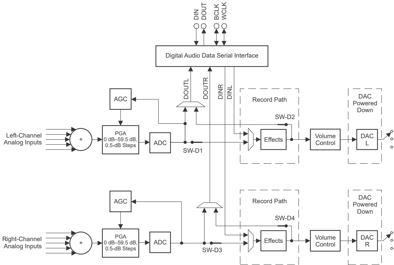
Figure 7-11. Record-Only Mode With Digital Processing Path Enabled
