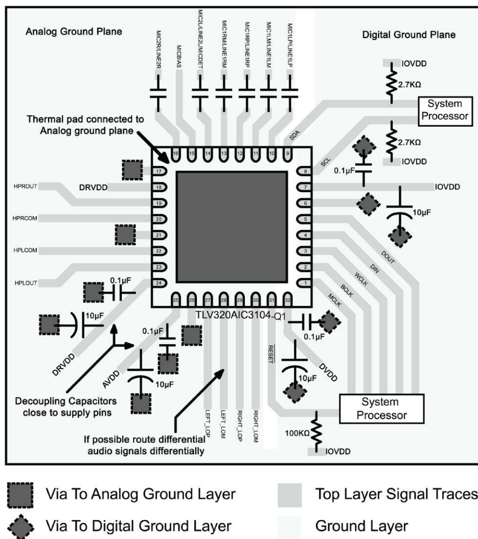
Figure 9-7. Layout Example
