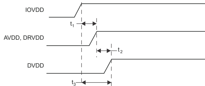
図 9-6. Power-Supply Sequencing
