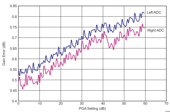
Figure 6-8. ADC Gain Error vs PGA Gain Setting
