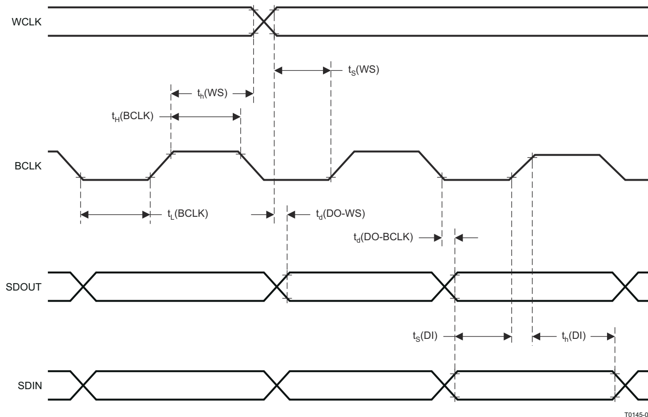
図 6-2. I²S/LJF/RJF Timing in Slave Mode
