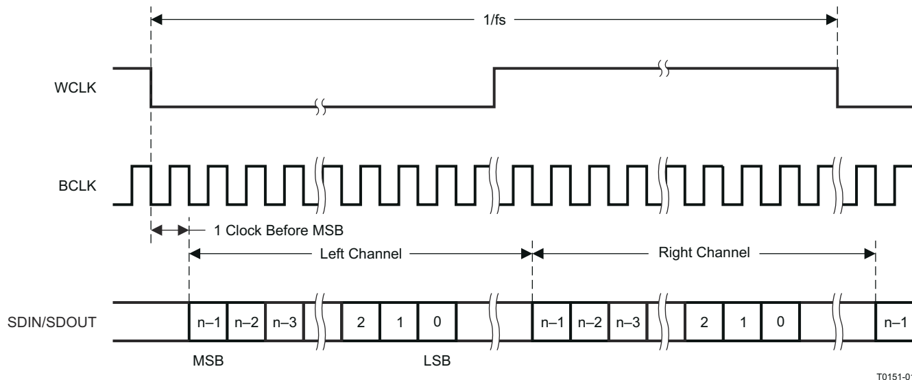
図 7-18. I 2 S Serial Data Bus Mode Operation
