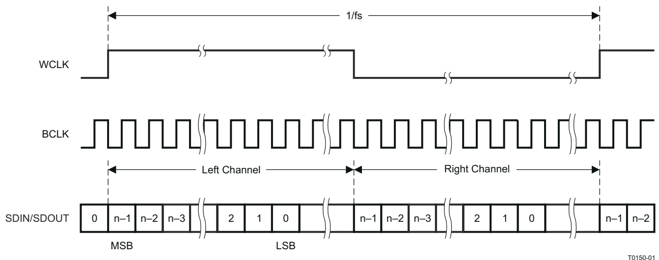
図 7-17. Left-Justified Serial Data Bus Mode Operation
