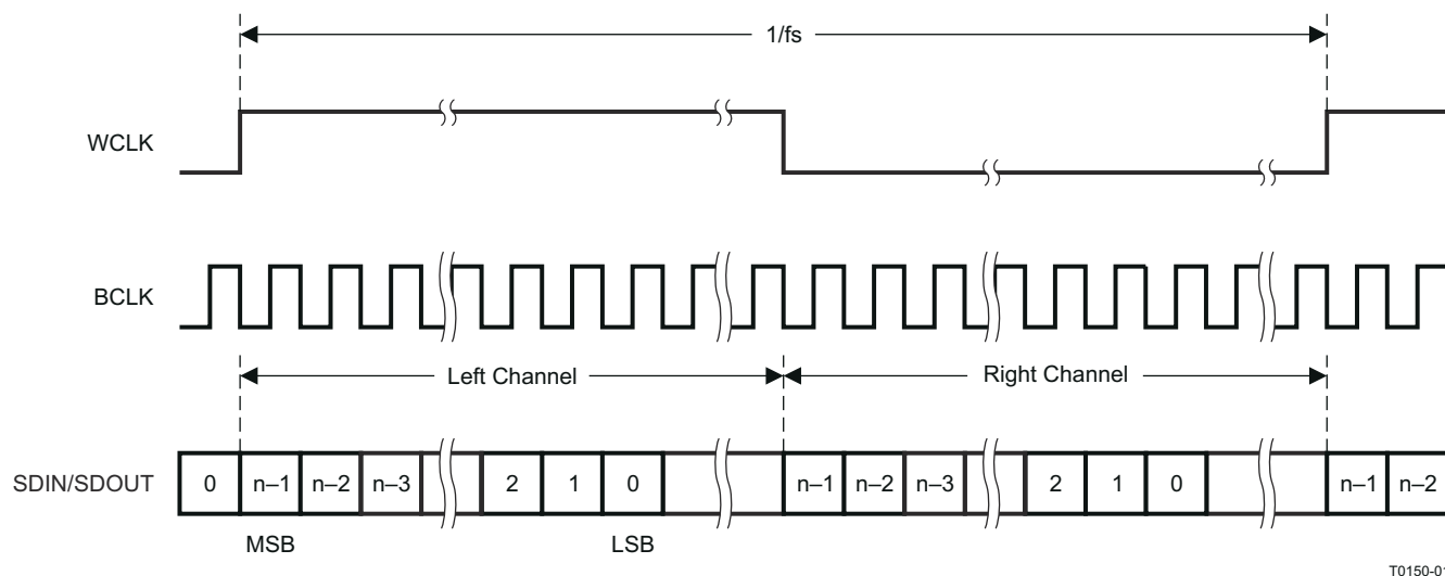
FIG 10-4. Left-Justified Serial Data Bus Mode Operation
