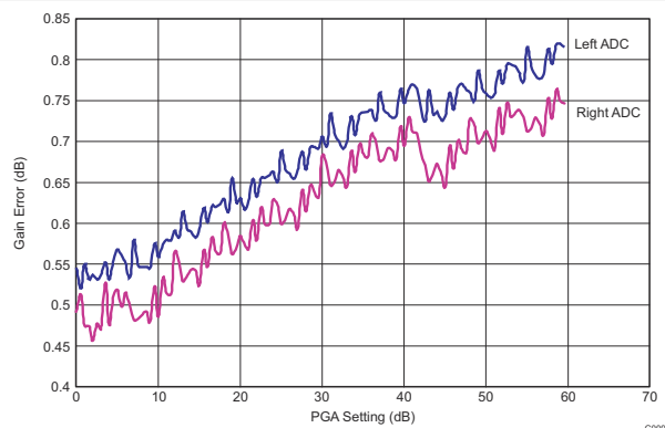
Figure 8-9. ADC Gain Error vs PGA Gain Setting
