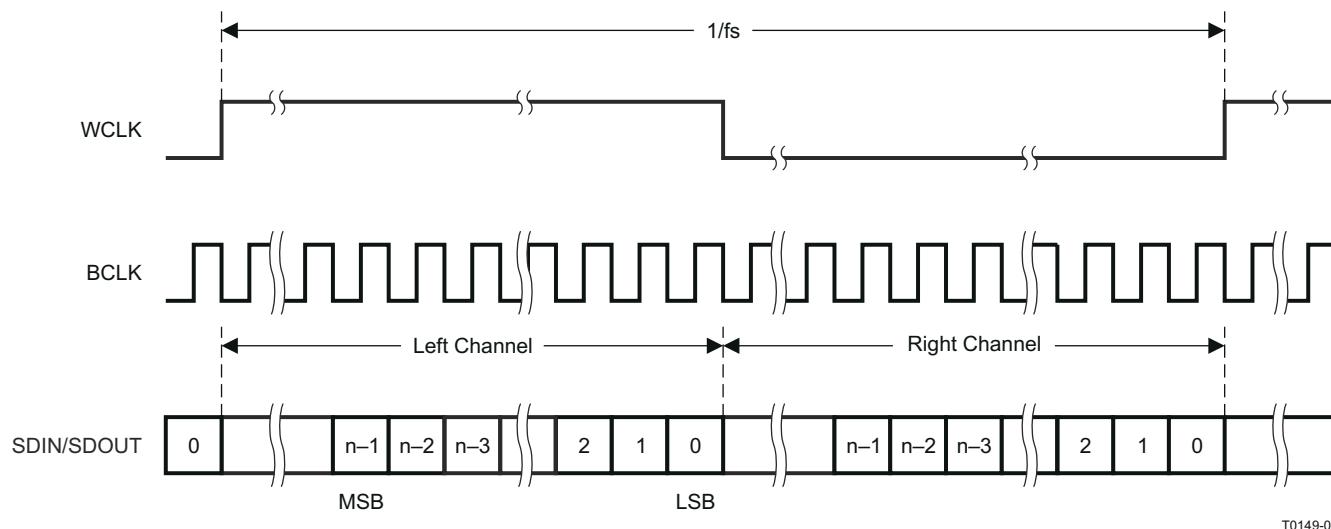
FIG 10-3. Right-Justified Serial Data Bus Mode Operation
