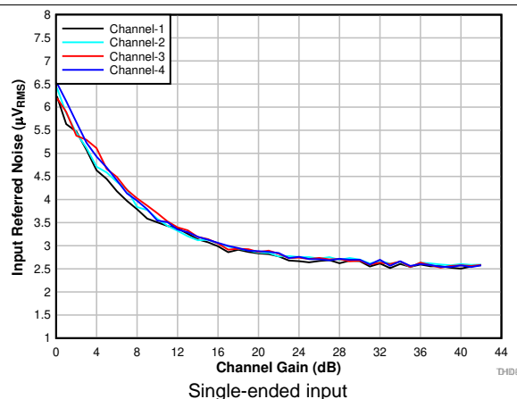
FIG 14. Input-Referred Noise vs Channel Gain
