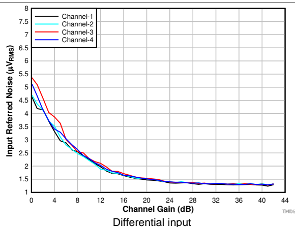
FIG 13. Input-Referred Noise vs Channel Gain
