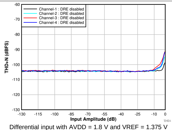
Figure 10. THD+N vs Input Amplitude With DRE Disabled
