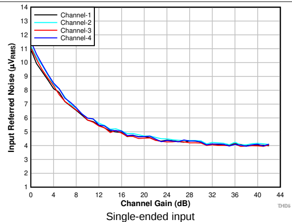
FIG 14. Input-Referred Noise vs Channel Gain Single-ended input
