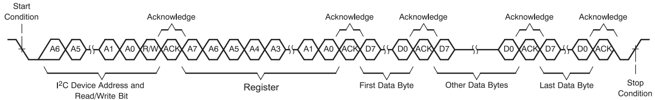
❏ 90. I 2 C Multiple-Byte Write Transfer
