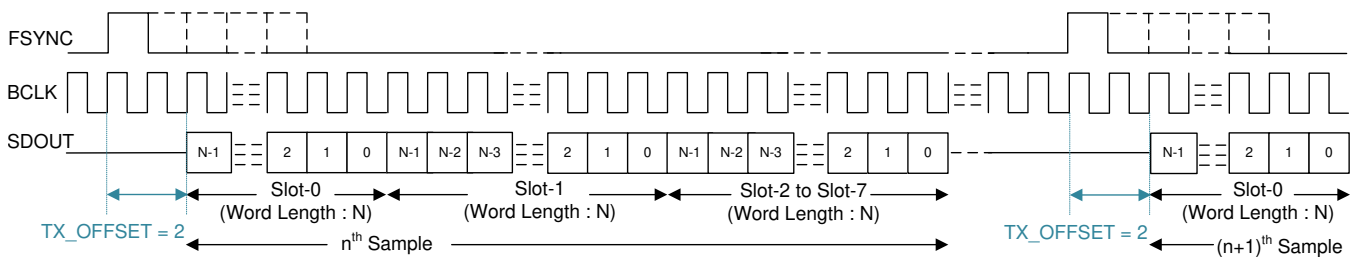
図 24. TDM Mode Protocol Timing (TX_OFFSET = 2)
