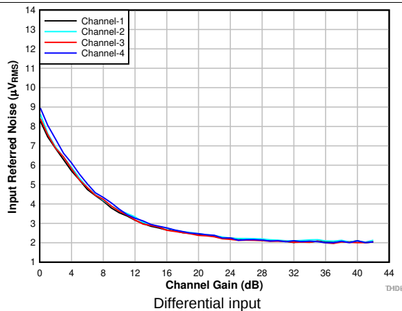
FIG 13. Input-Referred Noise vs Channel Gain Differential input
