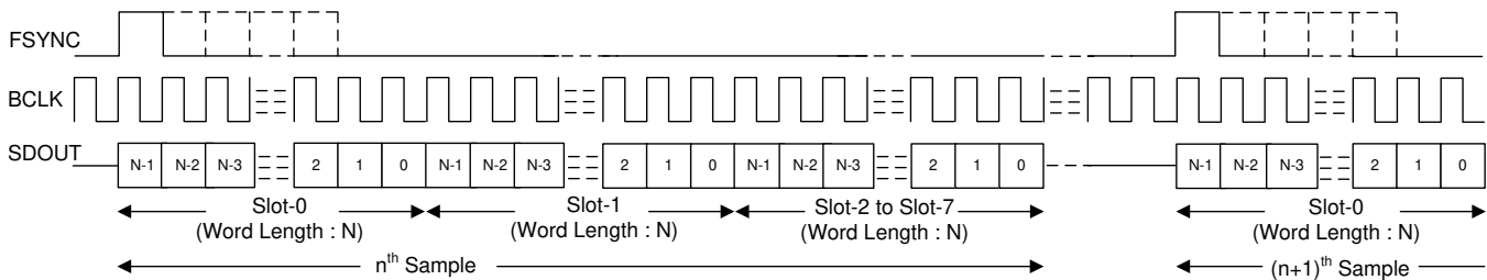
図 23. TDM Mode Standard Protocol Timing (TX_OFFSET = 0)
