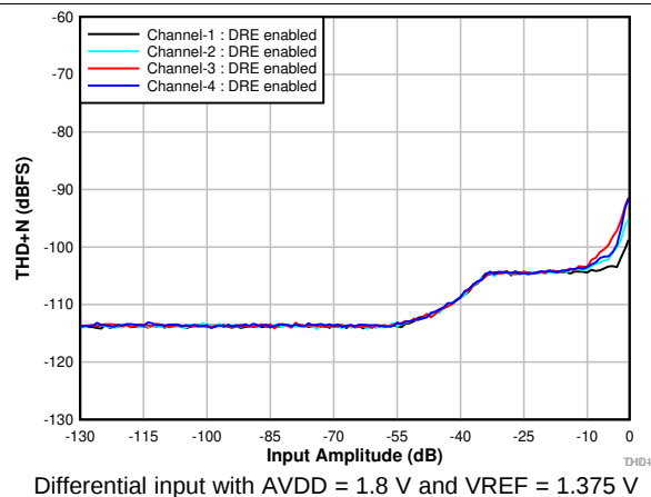
Figure 9. THD+N vs Input Amplitude With DRE Enabled
