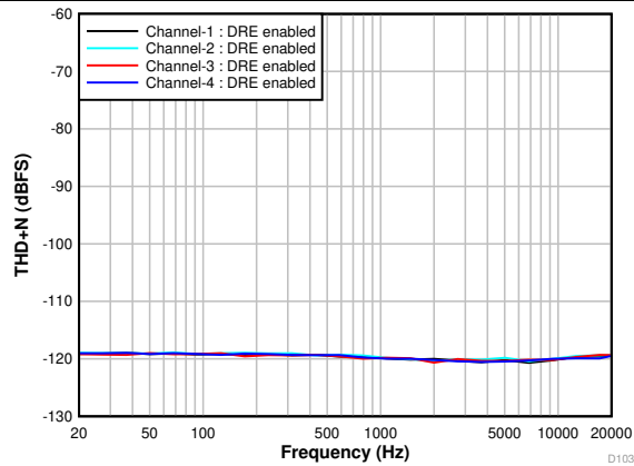
FIG 11. THD+N vs Input Frequency With a -60-dBr Input
