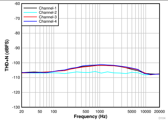
FIG 12. THD+N vs Input Frequency With a -1-dBr Input
