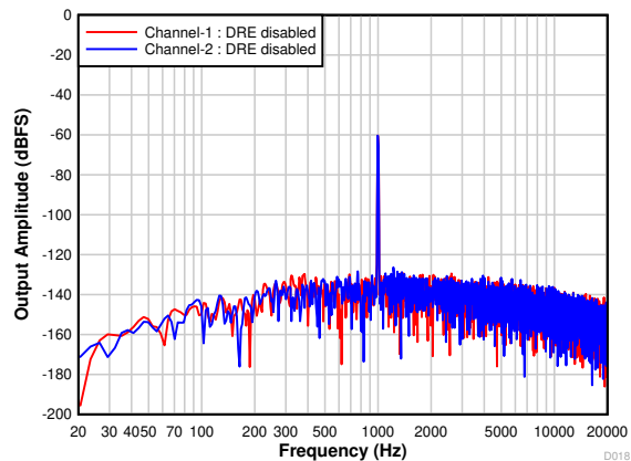
7-21. FFT With a -60-dBr Input With DRE Disabled
