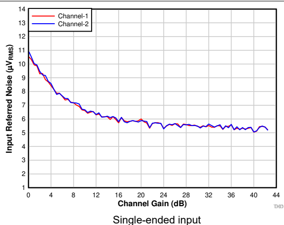
7-14. Input-Referred Noise vs Channel Gain
