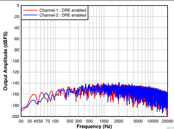
7-18. FFT With Idle Input With DRE Enabled
