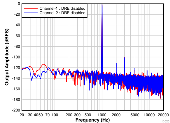
7-23. FFT With a -1\text{-dBr} Input With DRE Disabled
