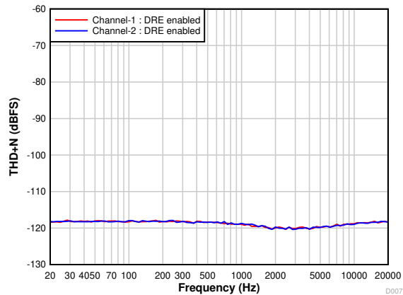
7-10. THD+N vs Input Frequency With a -60-dBr Input
