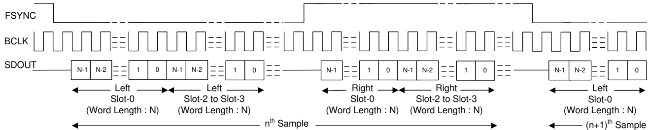
FIG 8-5. I 2 S Mode Standard Protocol Timing (TX_OFFSET = 0)
