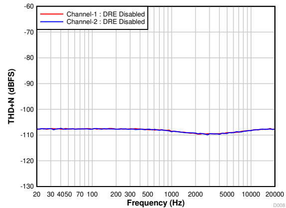
7-11. THD+N vs Input Frequency With a -60-dBr Input
