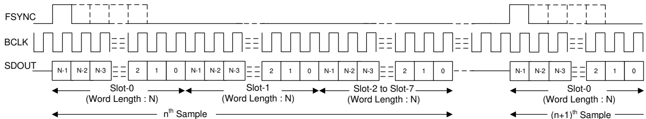
FIG 8-4. TDM Mode Protocol Timing (TX_OFFSET = 0 and BCLK_POL = 1)
