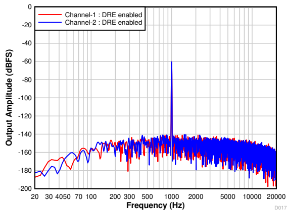
7-20. FFT With a -60-dBr Input With DRE Enabled
