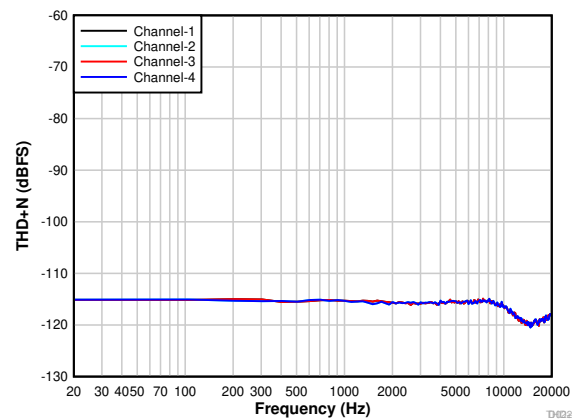
7-25. PDM Input THD+N vs Input Frequency With a -20\text{-dBr} Input
