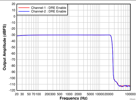
7-16. Frequency Response With a -30-dBr Input
