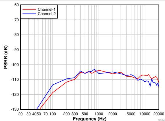
7-17. Power-Supply Rejection Ratio vs Ripple Frequency With 100-mV pp Amplitude
