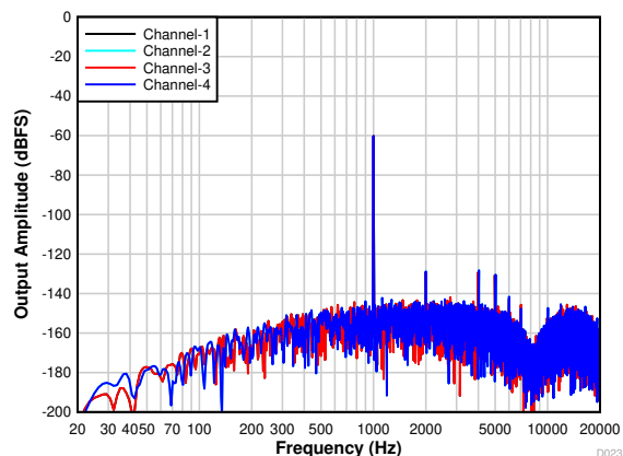
7-26. PDM Input FFT With a -60\text{-dBr} Input
