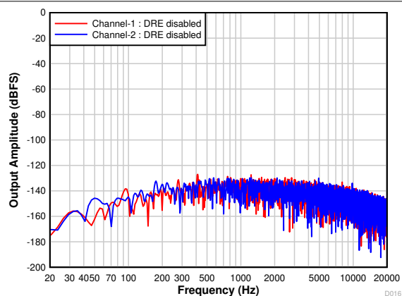
7-19. FFT With Idle Input With DRE Disabled
