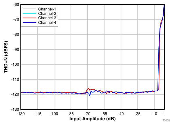
7-24. PDM Input THD+N vs Input Amplitude
