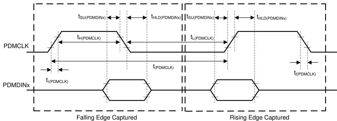
7-3. PDM Digital Microphone Interface Timing Diagram
