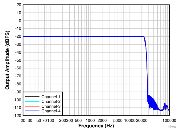
7-27. PDM Input Frequency Response With a -20\text{-dBr} Input
