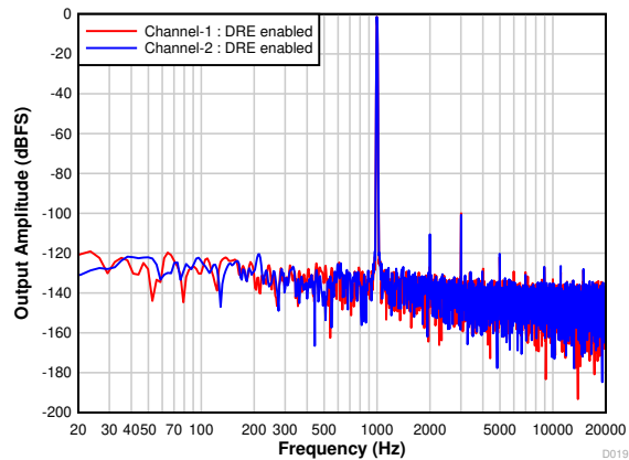
7-22. FFT With a -1\text{-dBr} Input With DRE Enabled
