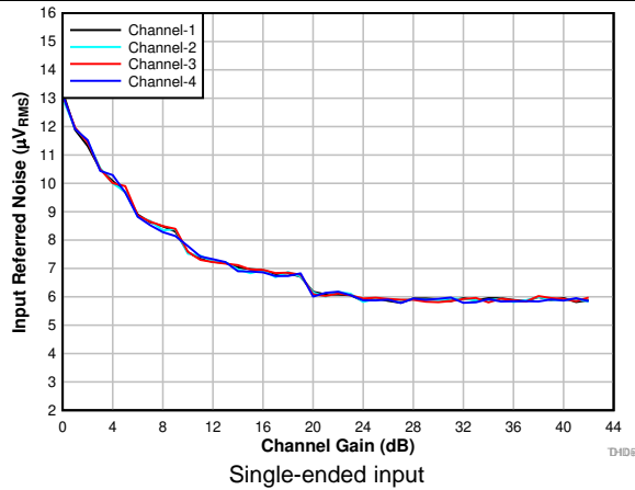
FIG 11. Input-Referred Noise vs Channel Gain
