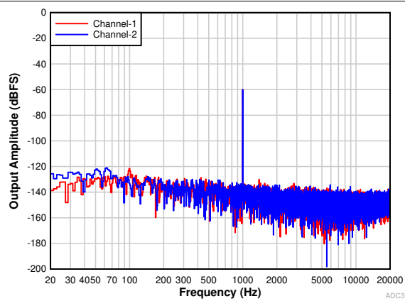
图 9-2. FFT With a -60-dBr Input
