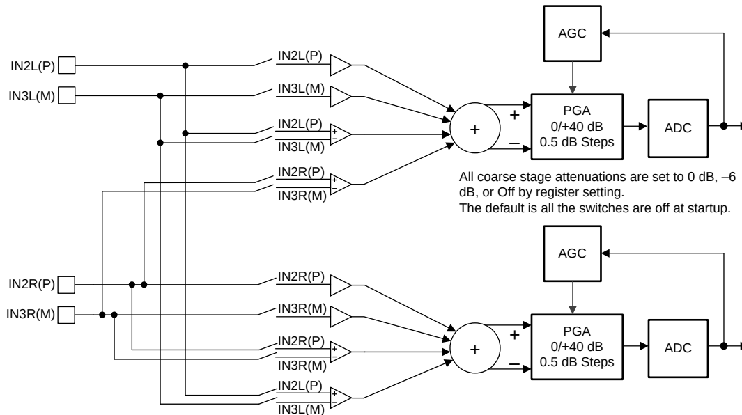
图 29. TLV320ADC3100 Available Audio Input Path Configurations
