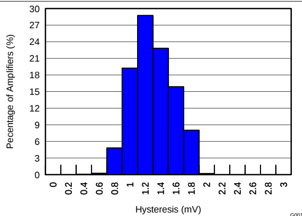
Figure 2. Hysteresis Distribution
