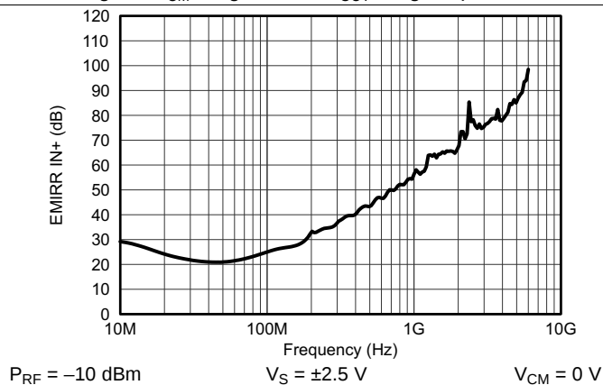
FIG 13. Electromagnetic Interference Rejection Ratio Referred to Noninverting Input (EMIRR IN+) vs Frequency
