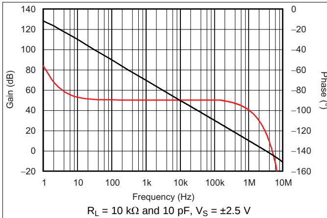
图 1. Open-Loop Gain and Phase vs Frequency
