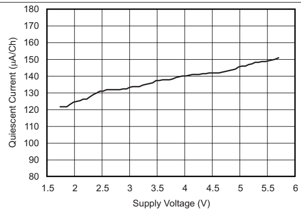
图 2. Quiescent Current vs Supply
