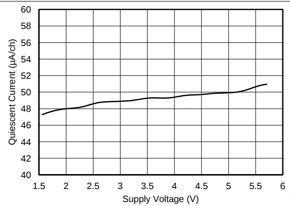
图 2. Quiescent Current vs Supply
