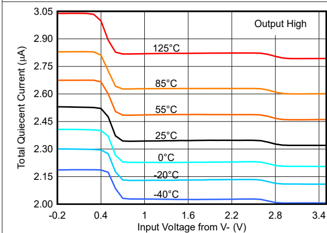
Figure 6-9. Supply Current vs. Common Mode - 3.3V
