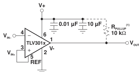
図 10-1. Basic Connections
