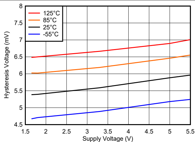
8-25. Hysteresis Voltage vs. Supply Voltage
