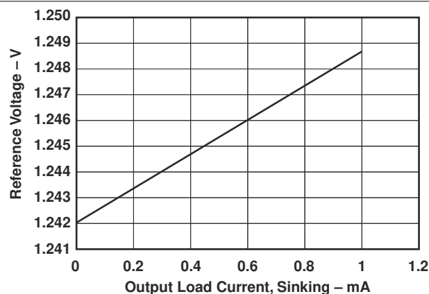
7-17. Reference Voltage vs Output Load Current (Sinking)
