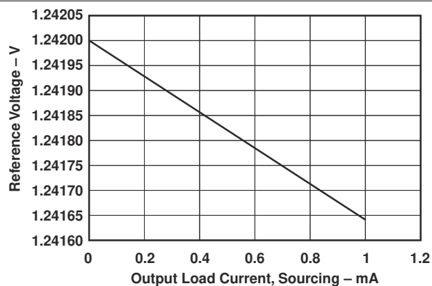
7-16. Reference Voltage vs Output Load Current (Sourcing)
