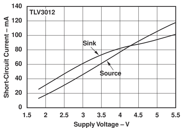
FIG 7-19. Short-Circuit Current vs Supply Voltage
