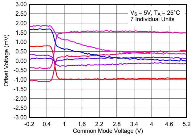
8-31. Offset Voltage vs. Common Mode Voltage, 5 V
