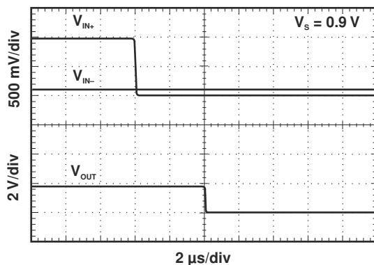
7-15. Propagation Delay ( t_{PHL} )
