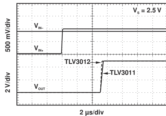
FIG 7-12. Propagation Delay ( t_{PLH} )
