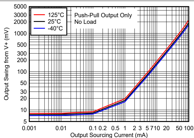
8-6. Output Swing vs. Output Sourcing Current - 5V
