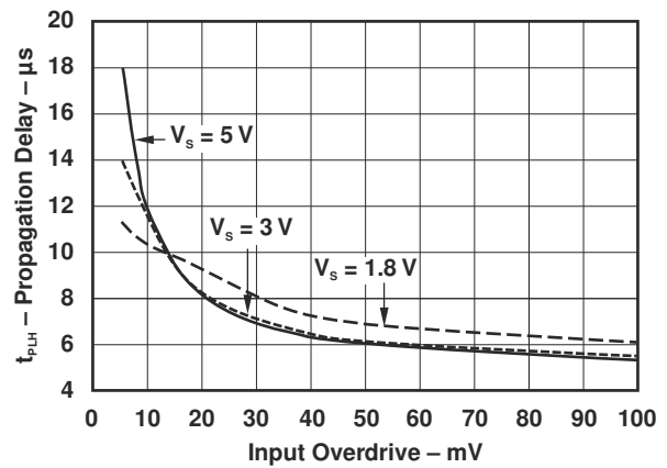
FIG 7-8. Propagation Delay ( t_{PLH} ) vs Input Overdrive
