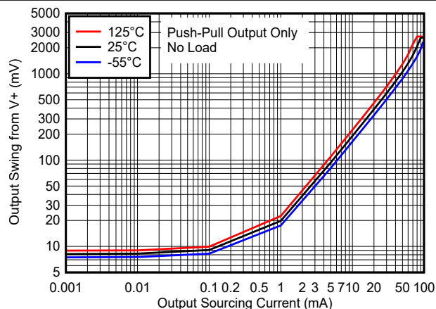
8-4. Output Swing vs. Output Sourcing Current - 3.3V
