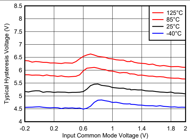
FIG 8-22. Hysteresis Voltage vs. Common Mode, 1.8V
