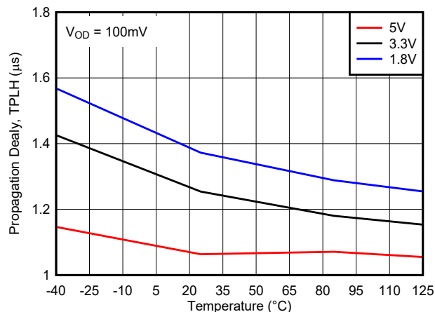
FIG 8-15. Low to High Propagation Delay vs. Temperature
