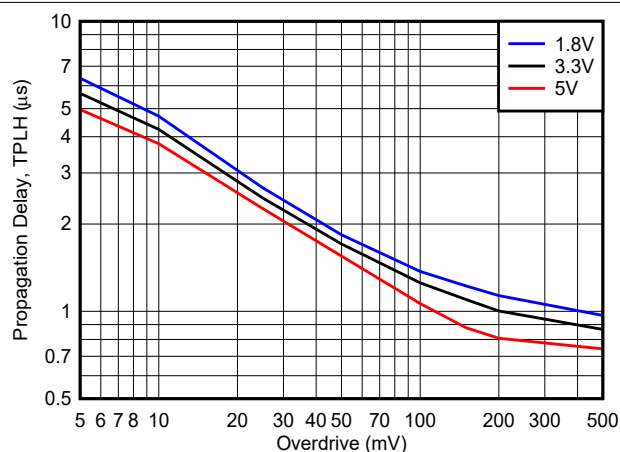
FIG 8-13. Low to High Propagation Delay vs. Overdrive
