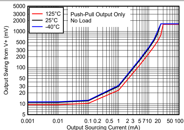
8-2. Output Swing vs. Output Sourcing Current - 1.8V
