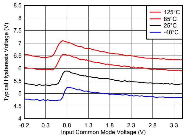
FIG 8-23. Hysteresis Voltage vs. Common Mode, 3.3V
