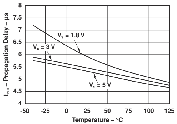
FIG 7-10. Propagation Delay ( t_{PLH} ) vs Temperature
