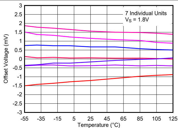
8-26. Offset Voltage vs. Temperature, 1.8 V
