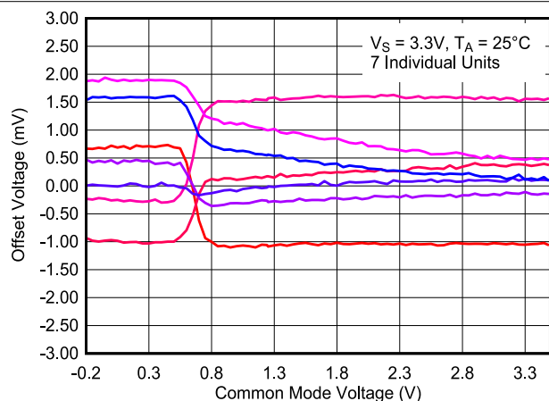
8-30. Offset Voltage vs. Common Mode Voltage, 3.3 V
