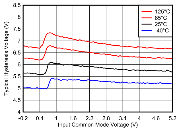
FIG 8-24. Hysteresis Voltage vs. Common Mode, 5V
