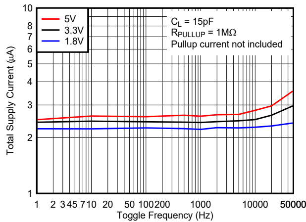
FIG 8-19. Supply Current vs. Toggle Frequency - Open Drain Output
