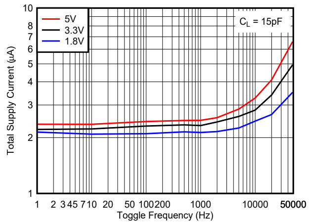
FIG 8-20. Supply Current vs. Toggle Frequency - Push-Pull Output
