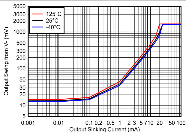
8-1. Output Swing vs. Output Sinking Current - 1.8V
