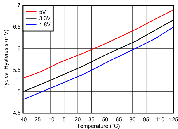
FIG 8-21. Hysteresis Voltage vs. Temperature
