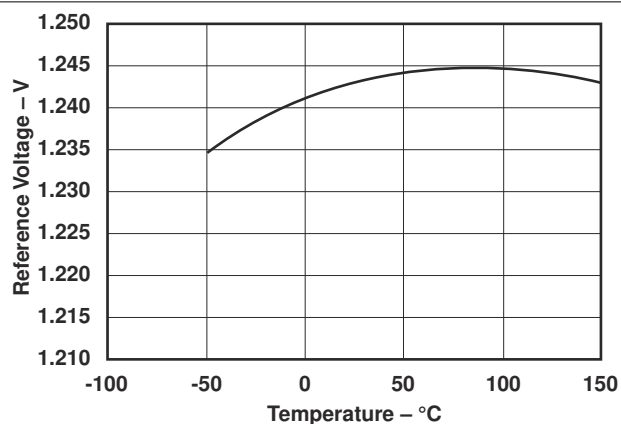
7-18. Reference Voltage vs Temperature
