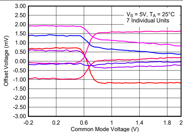
8-29. Offset Voltage vs. Common Mode Voltage, 1.8 V
