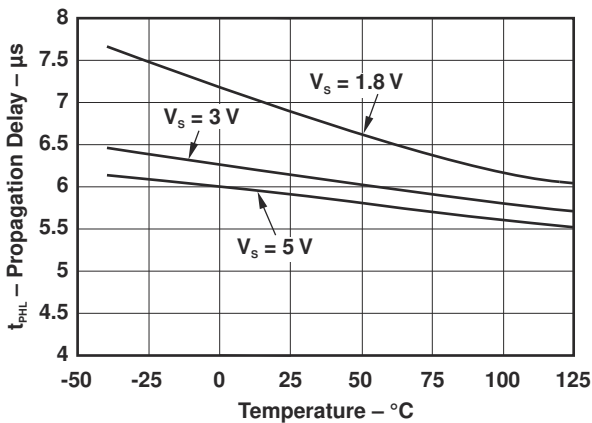
FIG 7-11. Propagation Delay ( t_{PHL} ) vs Temperature
