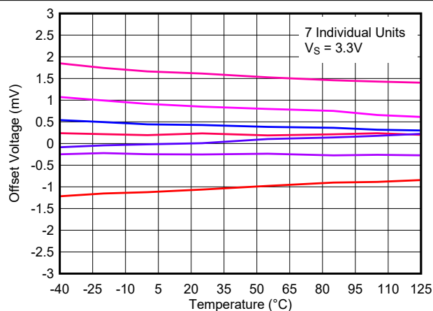
8-27. Offset Voltage vs. Temperature, 3.3 V
