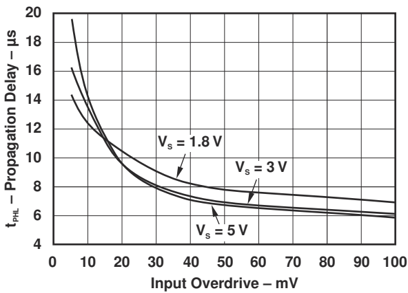
FIG 7-9. Propagation Delay ( t_{PHL} ) vs Input Overdrive
