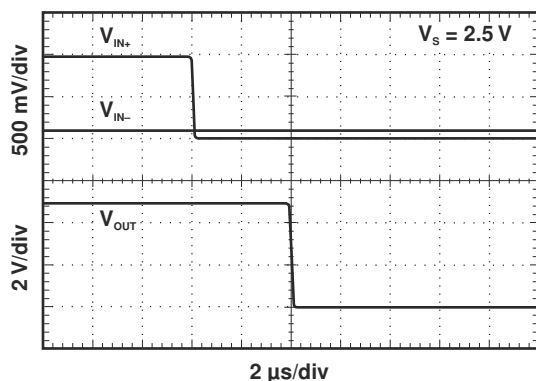
7-13. Propagation Delay ( t_{PHL} )
