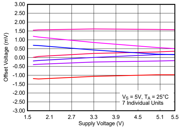
8-33. Offset Voltage vs. Supply Voltage, 25°C
