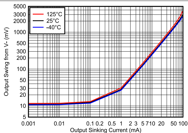
8-5. Output Swing vs. Output Sinking Current - 5V
