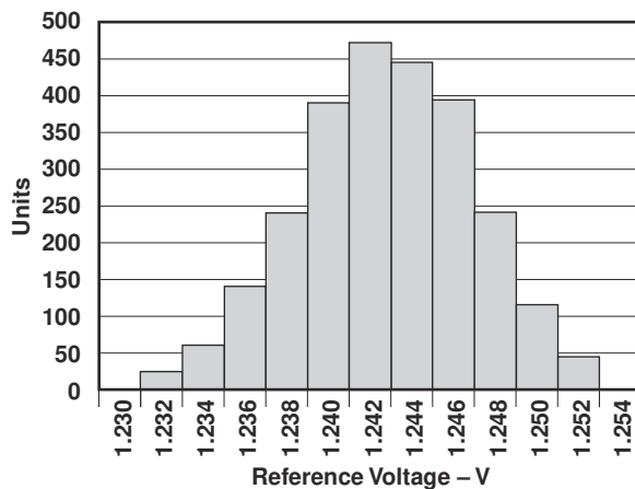
FIG 7-20. Reference Voltage Distribution
