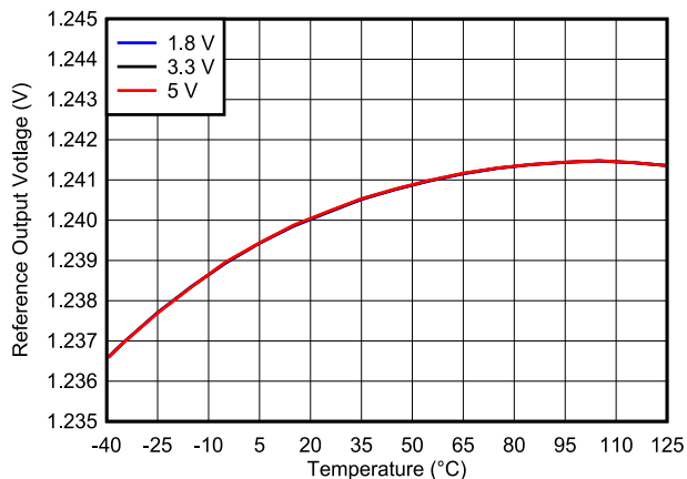
FIG 8-16. Reference Voltage vs. Temperature
