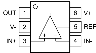
図 5-1. DCK, DBV Package 6-Pin SC-70, SOT-23 Top View
