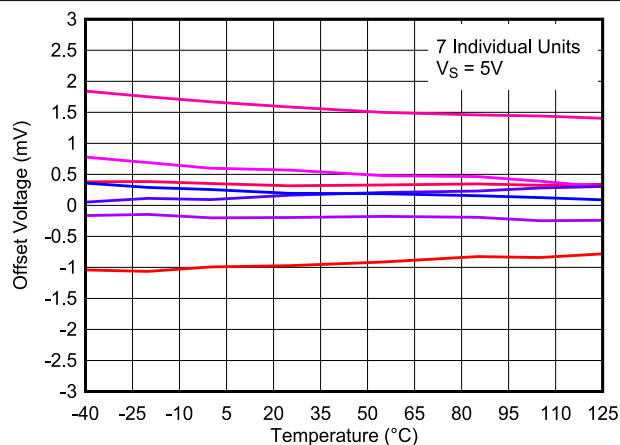
8-28. Offset Voltage vs. Temperature, 5 V
