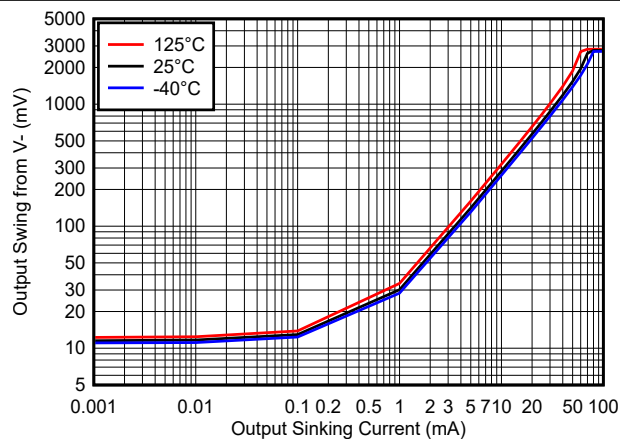
8-3. Output Swing vs. Output Sinking Current - 3.3V
