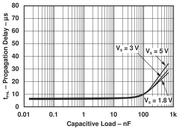
FIG 7-7. Propagation Delay ( t_{PHL} ) vs Capacitive Load
