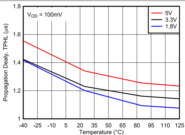
FIG 8-14. High to Low Propagation Delay vs. Temperature
