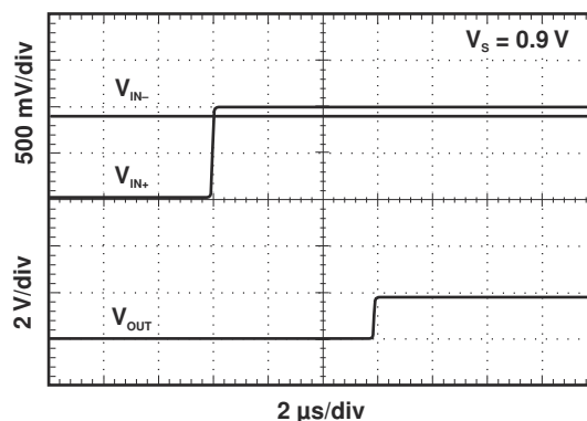
7-14. Propagation Delay ( t_{PLH} )
