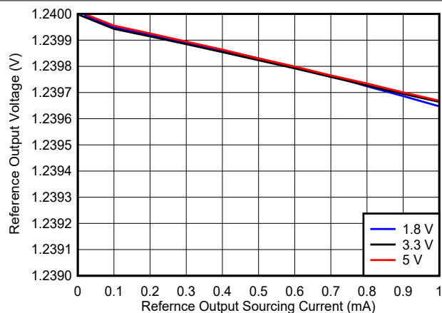
FIG 8-17. Reference Voltage vs. Reference Output Sourcing Current
