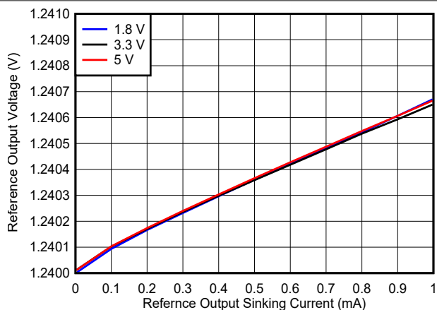
FIG 8-18. Reference Voltage vs. Reference Output Sinking Current
