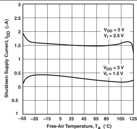
26. Shutdown Supply Current vs Free-Air Temperature
