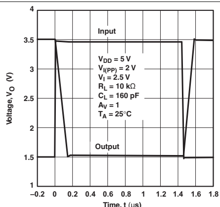
FIG 43. Small Signal Follower
