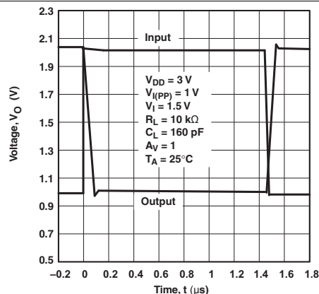
FIG 44. Inverting Large Signal
