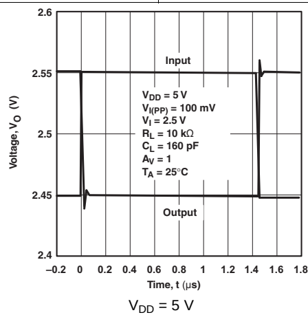
FIG 47. Inverting Small Signal
