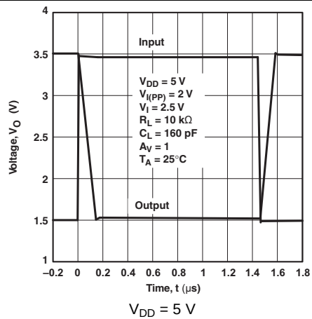
FIG 45. Inverting Large Signal
