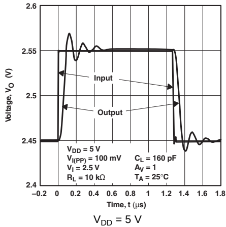
FIG 43. Small Signal Follower
