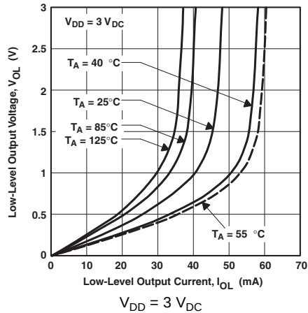
Figure 7. Low-Level Output Voltage vs Low-Level Output Current
