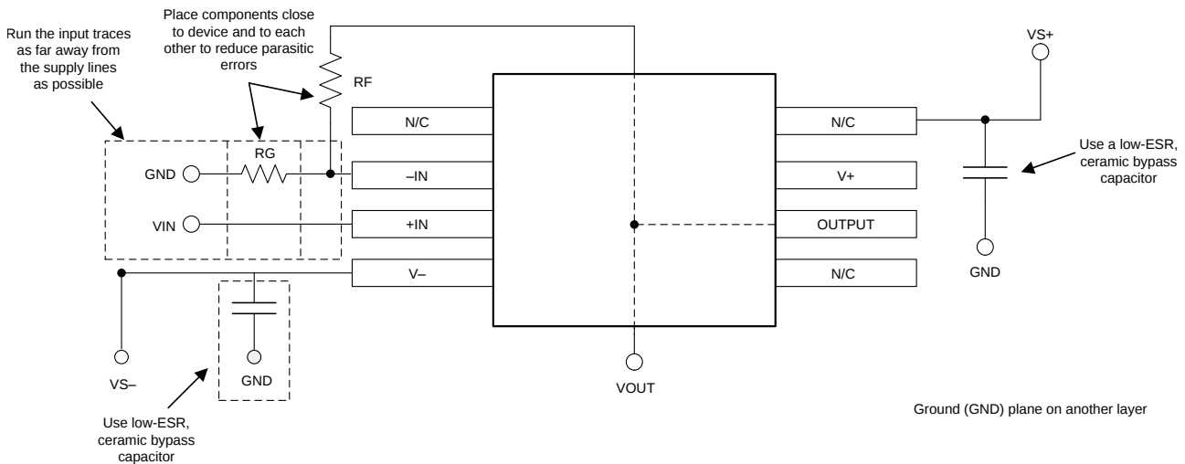
FIG 58. Operational Amplifier Board Layout for Noninverting Configuration
