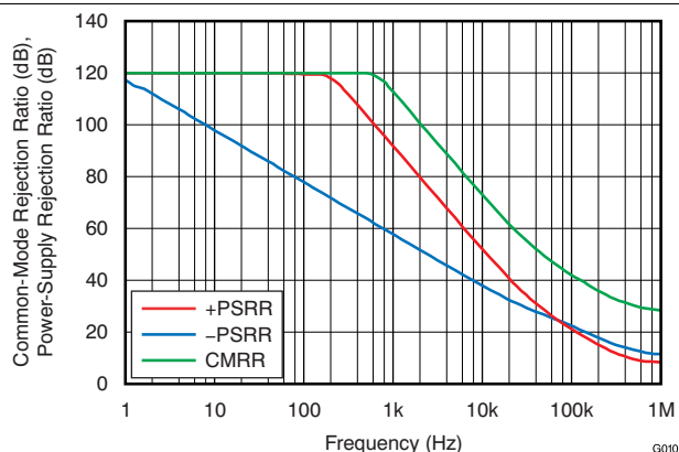
FIG 6. CMRR and PSRR vs Frequency (Referred-to Input)
