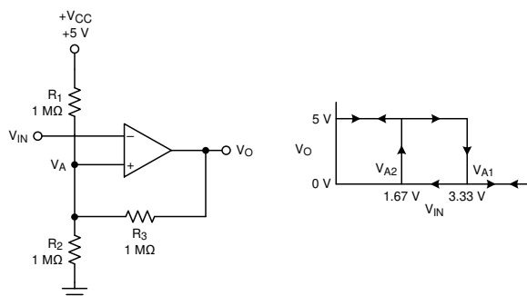
Figure 8-3. TLV185x-Q1 in an Inverting Configuration With Hysteresis
