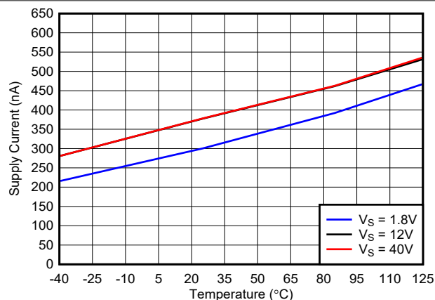
FIG 6-25. Supply Current vs. Temperature (Output Low), Open Drain
