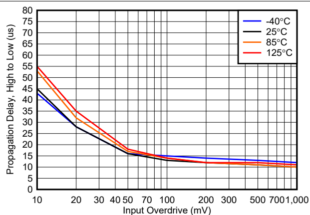
Figure 6-34. Propagation Delay, High to Low, 12 V
