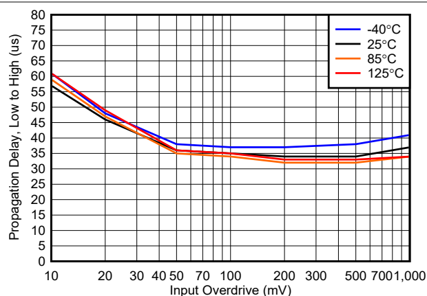
FIG 6-29. Propagation Delay, Low to High, 12 V, Open Drain
