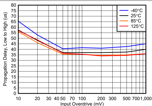
FIG 6-27. Propagation Delay, Low to High, 1.8 V, Open Drain
