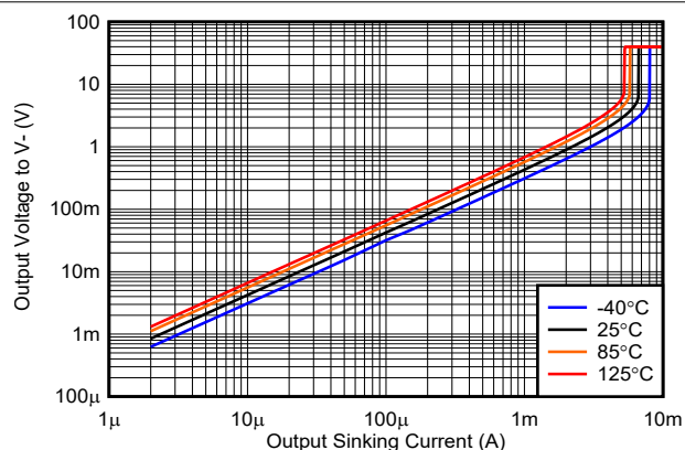
图 6-18. Output Voltage vs. Output Sinking Current, 40 V
