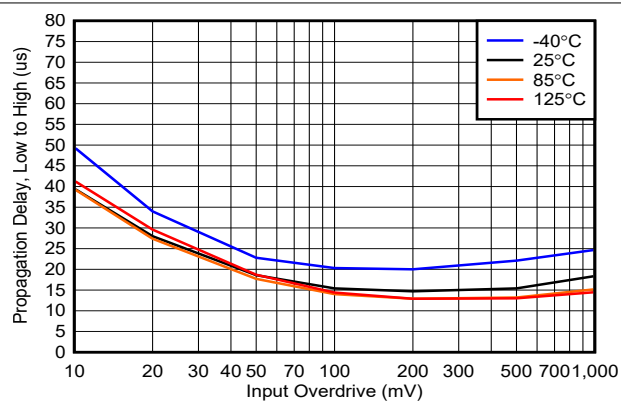
FIG 6-30. Propagation Delay, Low to High, 12 V, Push-Pull
