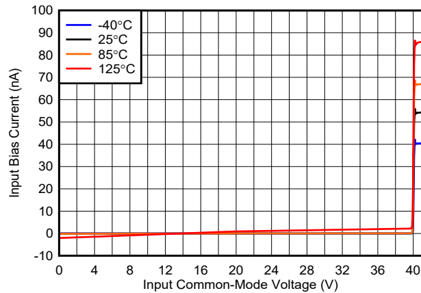
図 6-11. Bias Current vs. Common-Mode, 40 V
