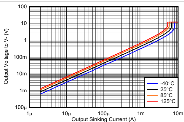
图 6-16. Output Voltage vs. Output Sinking Current, 12 V
