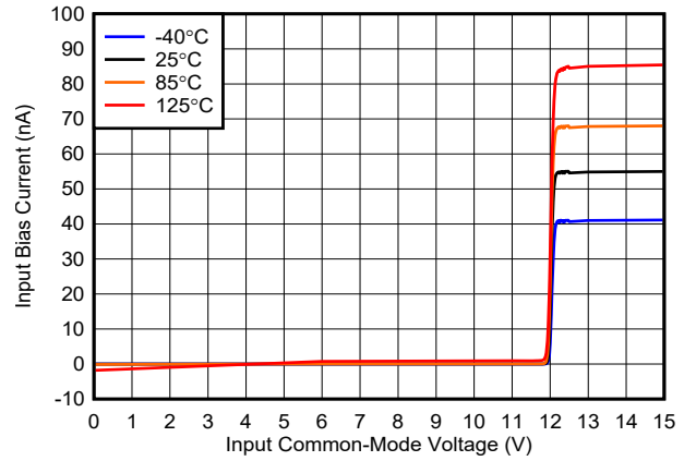
図 6-10. Bias Current vs. Common-Mode, 12 V
