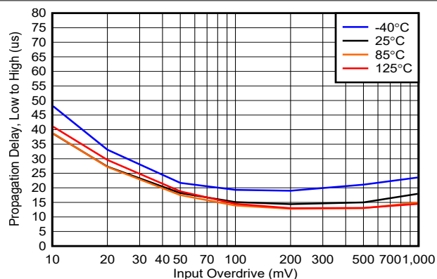
Figure 6-32. Propagation Delay, Low to High, 40 V, Push-Pull
