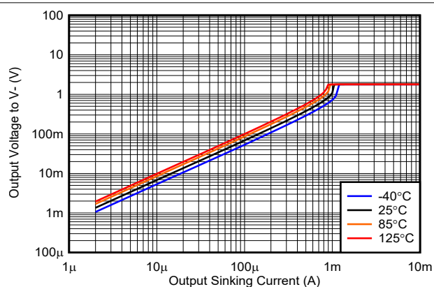
图 6-14. Output Voltage vs. Output Sinking Current, 1.8 V
