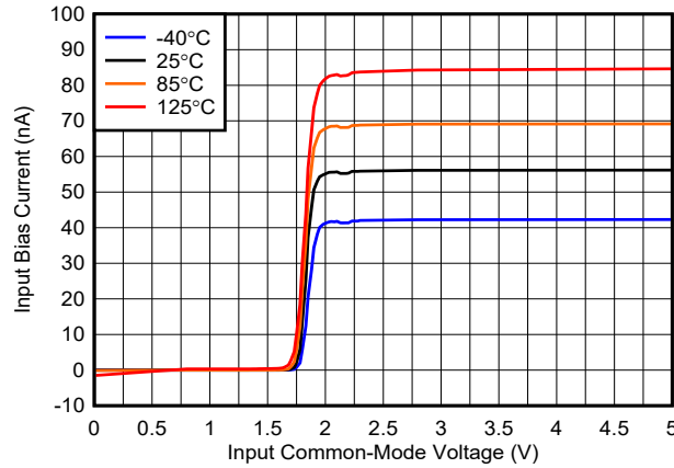
図 6-9. Bias Current vs. Common-Mode, 1.8 V
