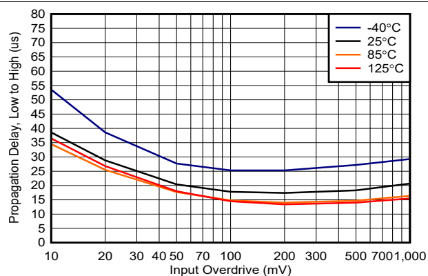
FIG 6-28. Propagation Delay, Low to High, 1.8 V, Push-Pull
