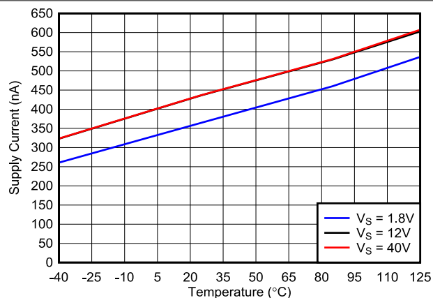
FIG 6-26. Supply Current vs. Temperature (Output High), Open Drain
