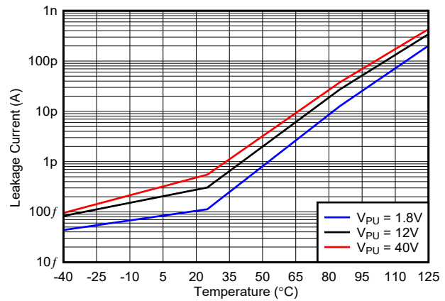
図 6-12. Leakage Current vs. Temperature (Open Drain only)
