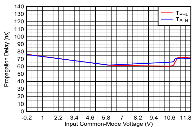
FIG 5-16. Propagation Delay vs. Common-Mode, 12V
