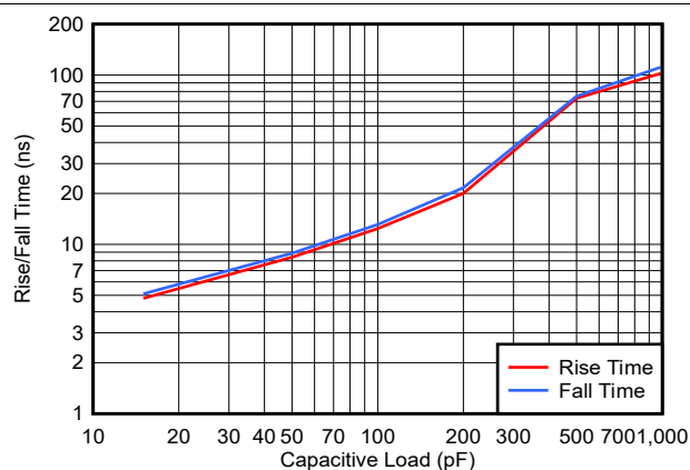
FIG 5-18. Rise/Fall Time vs. Capacitive Load, 12V
