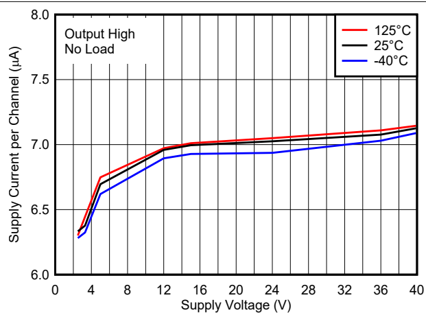
FIG 7-2. Supply Current per Channel vs. Supply Voltage, Output High
