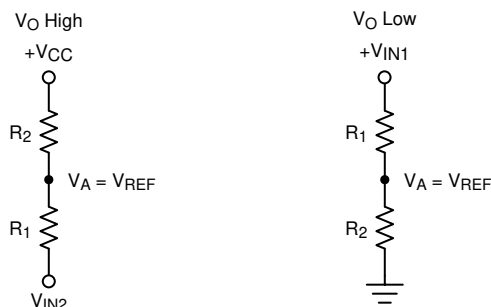
图 9-6. Non-Inverting Configuration Resistor Networks
