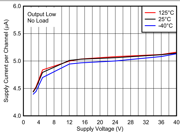
FIG 7-1. Supply Current per Channel vs. Supply Voltage, Output Low
