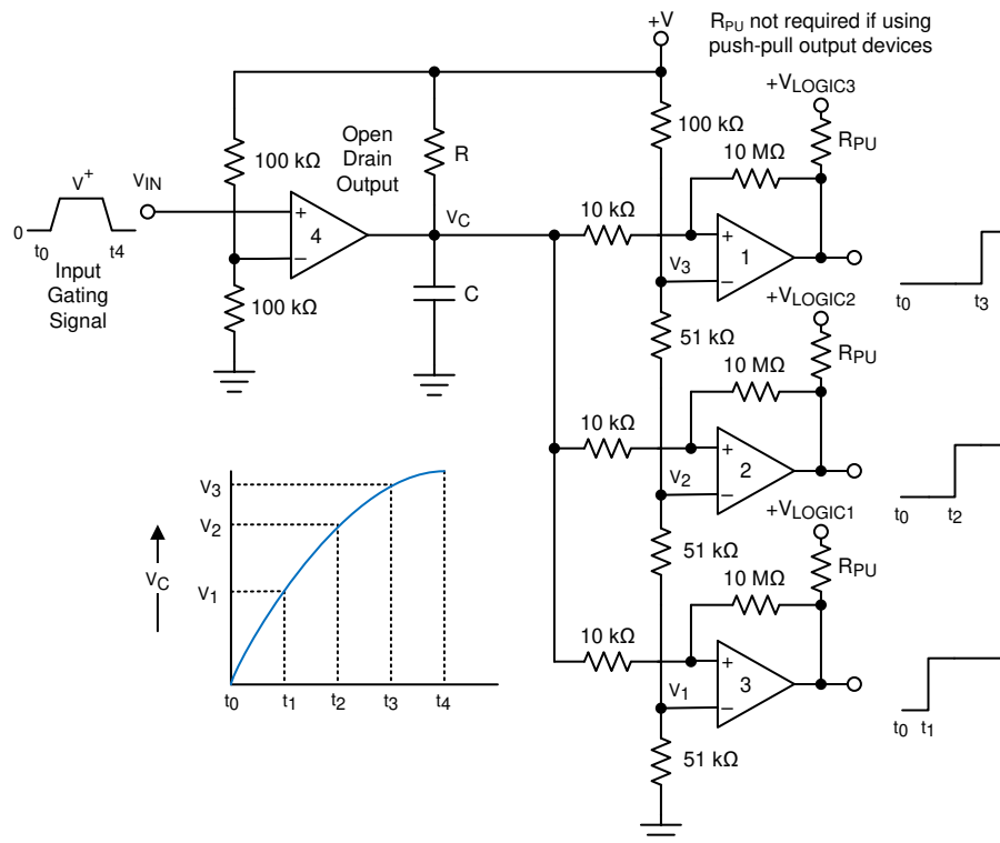
FIG 9-13. Time Delay Generator
