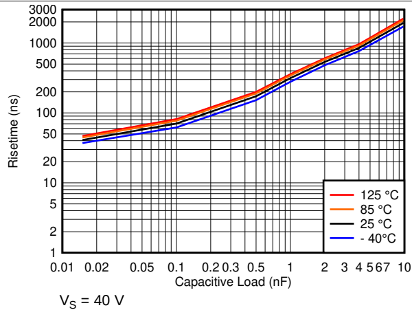
FIG 57. t_{\text{RISE}} vs. Capacitive Load at 40V
