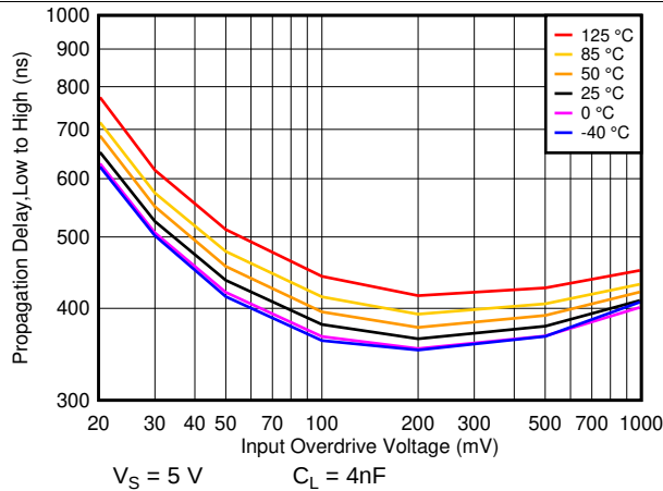
FIG 45. T_{PLH} Response Time vs. Overdrive at 5V
