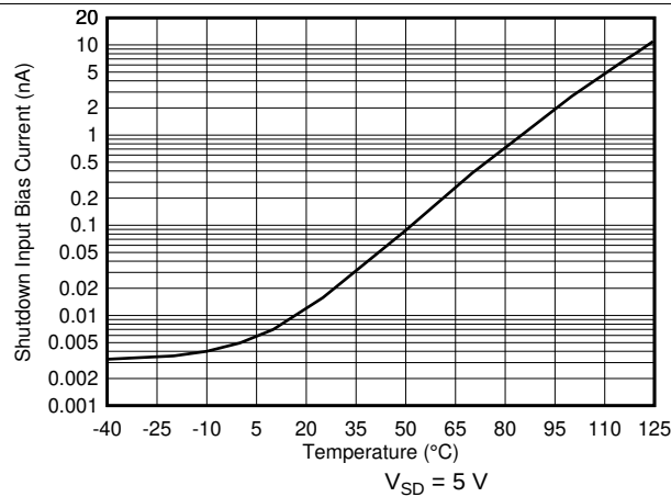
FIG 21. Shutdown Input Bias Current vs. Temperature
