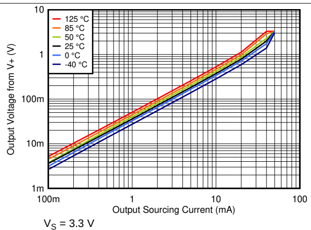
FIG 26. Output Sourcing Current vs. Output Voltage at 3.3V
