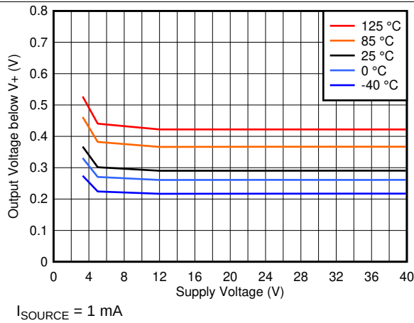
FIG 23. Output High Voltage vs. Supply Voltage
