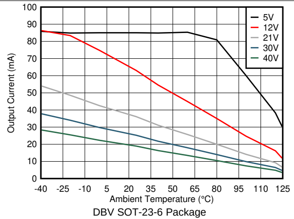
FIG 22. Maximum Output Current vs. Ambient Temperature
