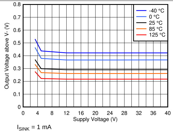
FIG 24. Output Low Voltage vs. Supply Voltage
