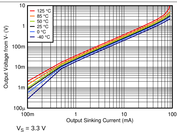
FIG 25. Output Sinking Current vs. Output Voltage at 3.3V
