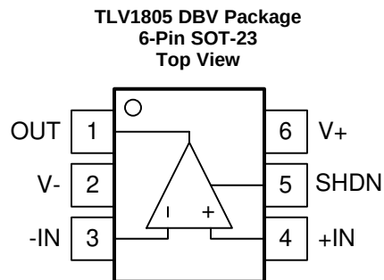
Pin Functions
