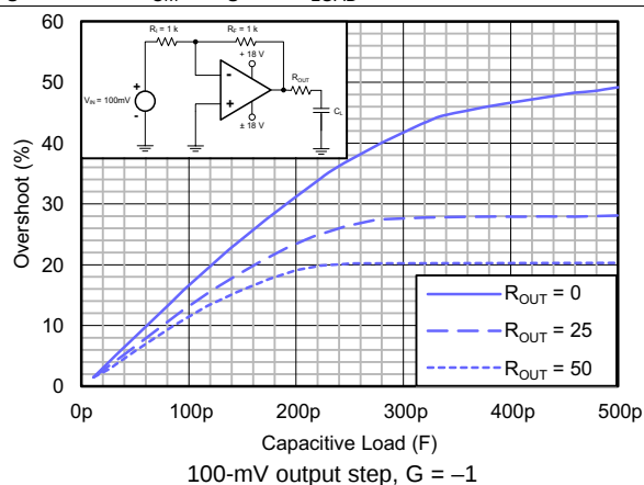
FIG 13. Small-Signal Overshoot vs Capacitive Load
