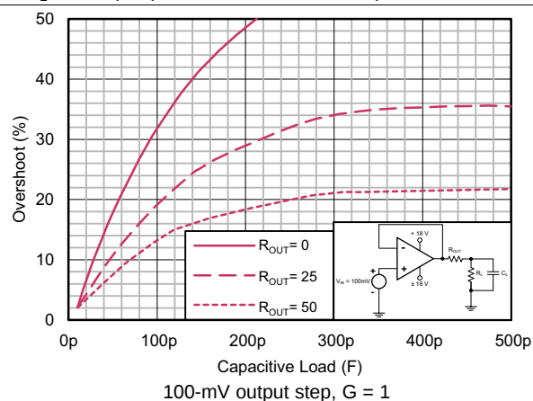
FIG 14. Small-Signal Overshoot vs Capacitive Load
