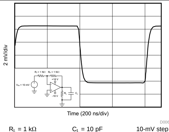
FIG 17. Small-Signal Step Response
