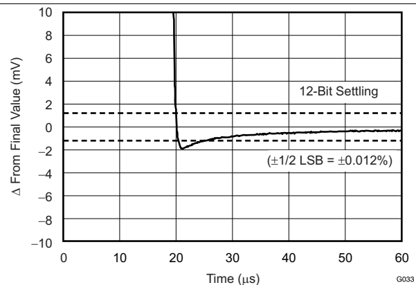
FIG 20. Large-Signal Step Response
