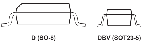
D (SO-8)
