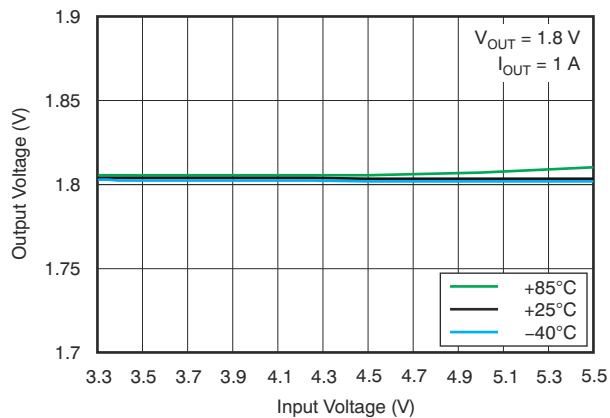
FIG 6-2. Line Regulation
