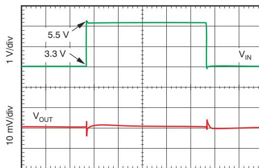
FIG 6-22. Line Transient Response
