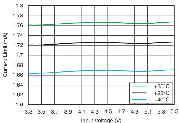
FIG 6-8. Current Limit vs Input Voltage
