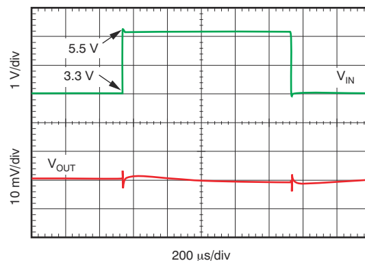
FIG 6-26. Line Transient Response
