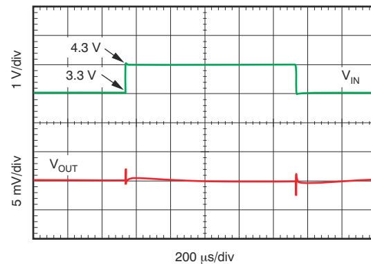
FIG 8-3. Line Transient Response V_{OUT} = 1.8\ \text{V} , I_{OUT} = 500\ \text{mA}
