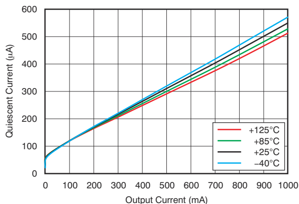
FIG 6-7. Quiescent Current vs Load
