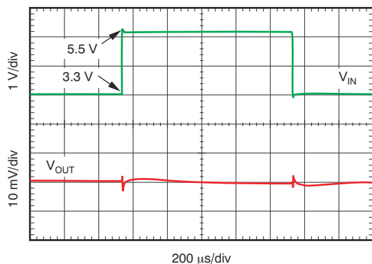
FIG 6-25. Line Transient Response
