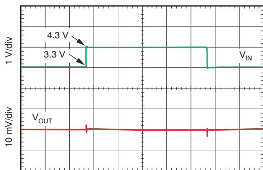
FIG 6-21. Line Transient Response
