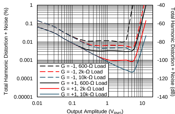
FIG 15. THD + N vs Output Amplitude
