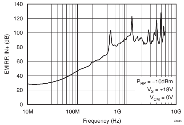
图 32. EMIRR IN+ vs Frequency
