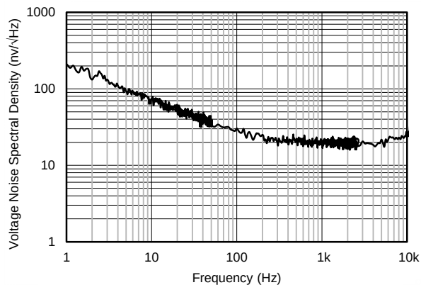
FIG 13. Input Voltage Noise Spectral Density vs Frequency
