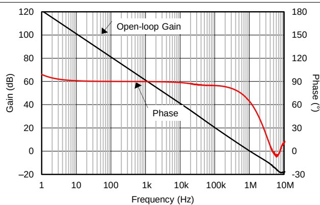
FIG 18. Open-Loop Gain and Phase vs Frequency
