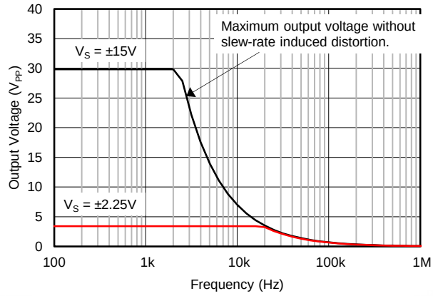
图 31. Maximum Output Voltage vs Frequency
