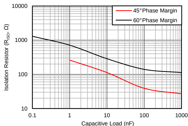
図 36. Isolation Resistor Required for Various Capacitive Loads to Achieve a Target Phase Margin
