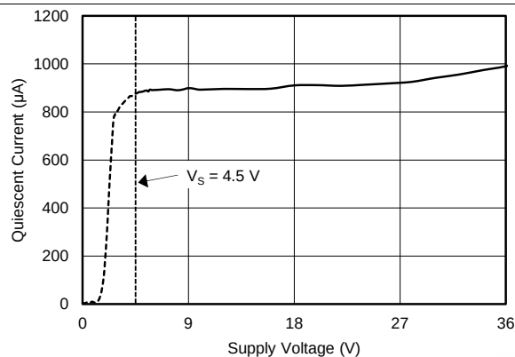
FIG 17. Quiescent Current vs Supply Voltage
