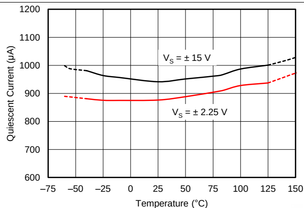
FIG 16. Quiescent Current vs Temperature
