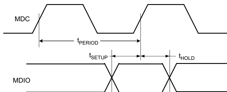
Figure 9-4. MDIO Read/Write Timing
