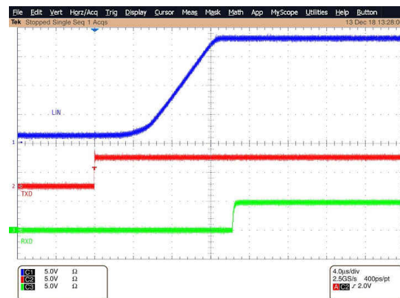
10-12. Dominant to Recessive Propagation Delay
