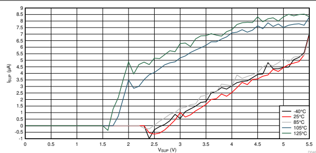
10-7. I_{SUP} vs V_{SUP} Across Temperature
