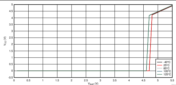
10-3. V_{CC} vs V_{SUP} Across Temperature
