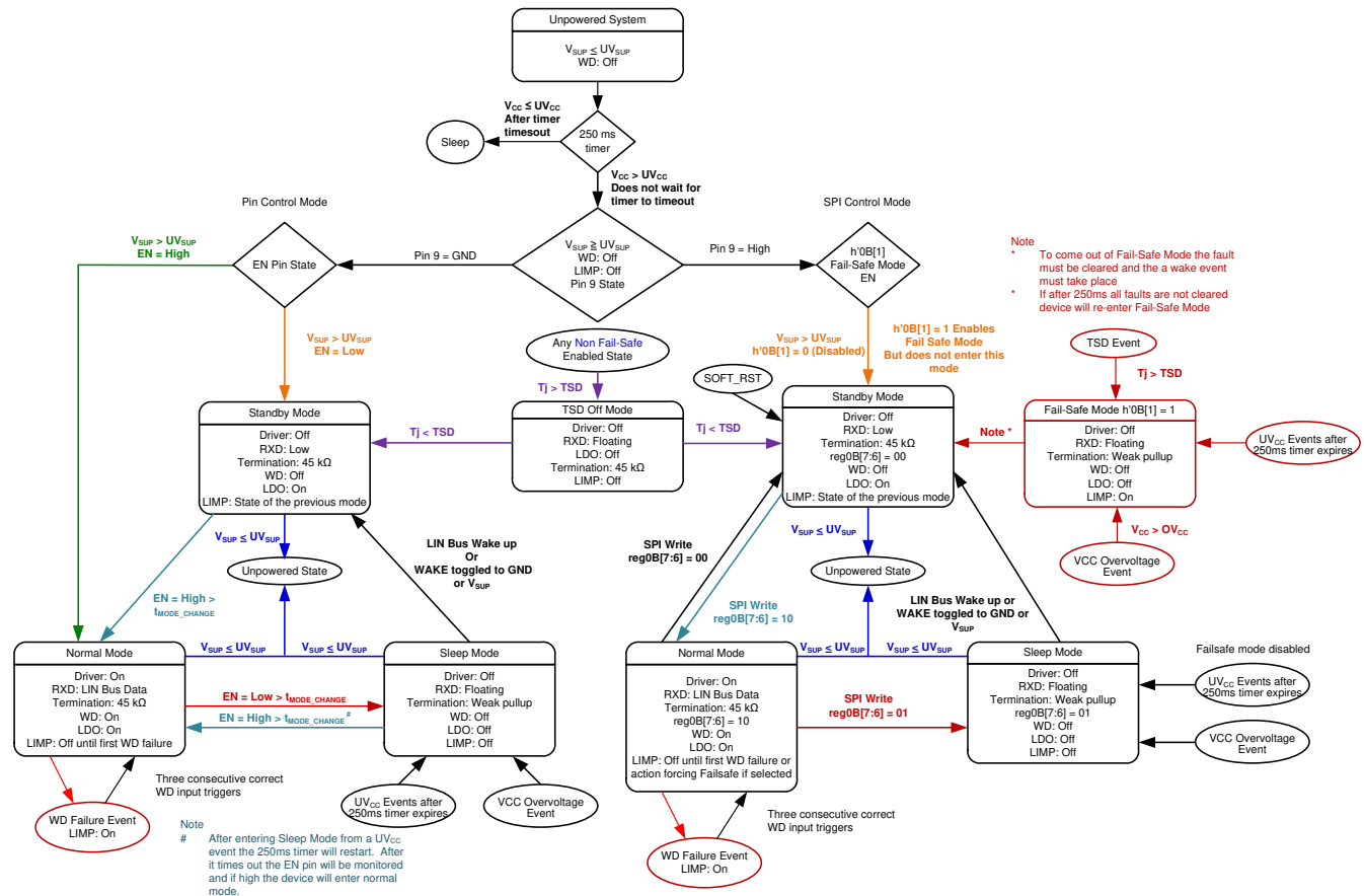
9-7. State Diagram with Failsafe
