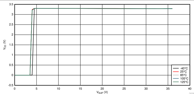
7-7. V_{CC} vs V_{SUP} Across Temperature
