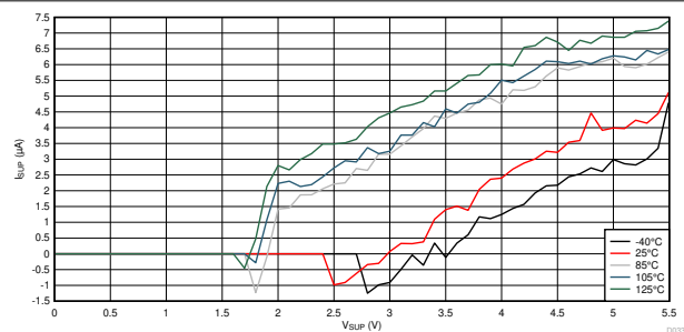
10-8. I_{SUP} vs V_{SUP} Across Temperature
