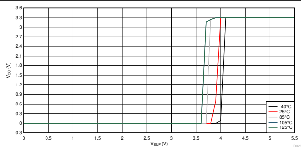
10-4. V_{CC} vs V_{SUP} Across Temperature
