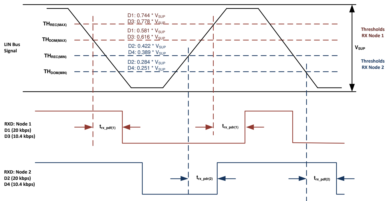
図 6-13. Propagation Delay
