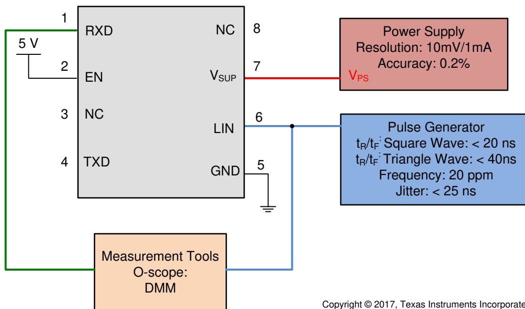
図 6-4. LIN Receiver Test with RX access Param 17, 18, 19, 20
