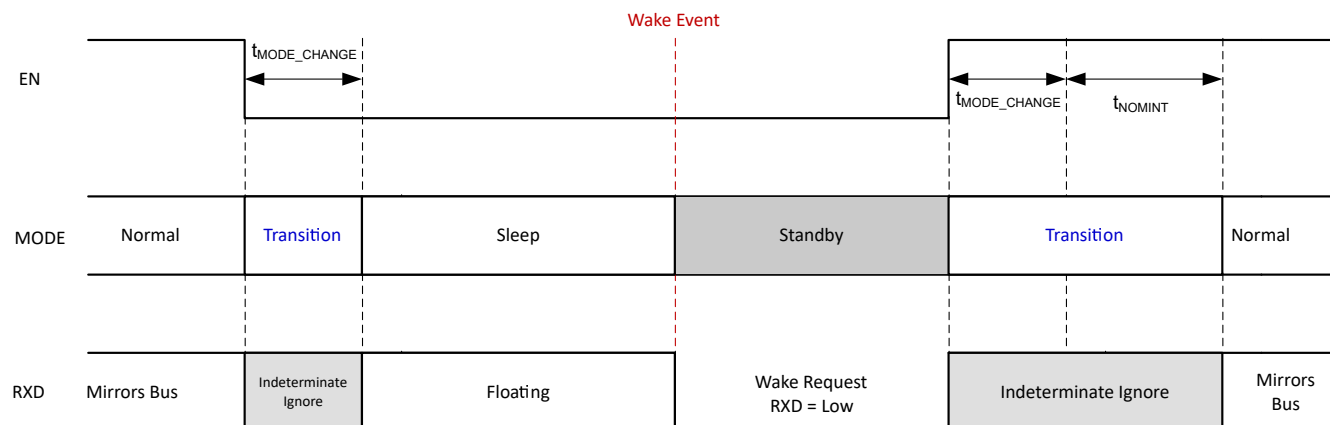
8-15. Mode Transitions
