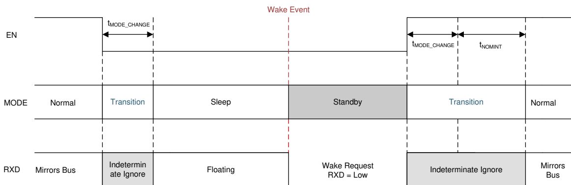
8-14. Mode Transitions
