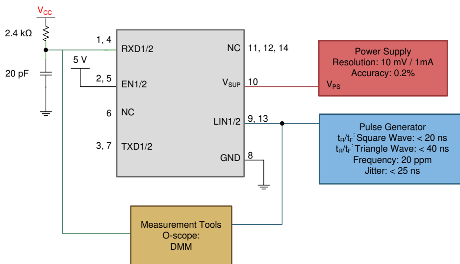
8-12. Propagation Delay Test Circuit; Parameters 31, 32
