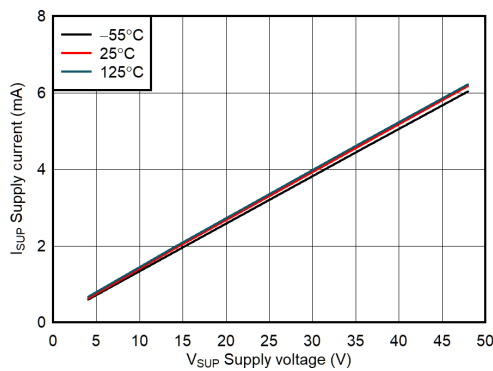
7-3. Supply Current vs Voltage Supply Across Temperature
