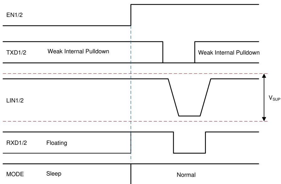
8-15. Wakeup Through EN
