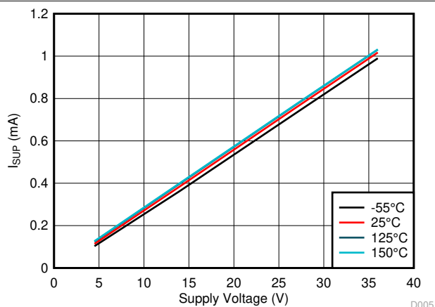
7-5. I_{SUP(STBY\_DOM)} vs V_{SUP} vs Temperature
