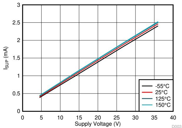
7-3. I_{SUP(DOM)} vs V_{SUP} vs Temperature
