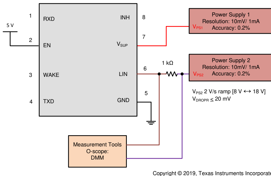
8-7. Test Circuit for I_{BUS\_PAS\_rec} Param 14
