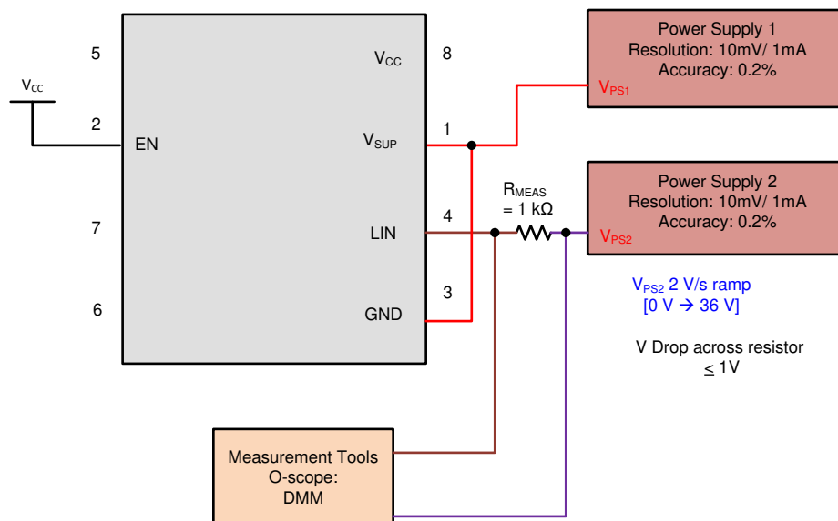
8-8. Test Circuit for I_{BUS\_NO\_GND} Loss of GND
