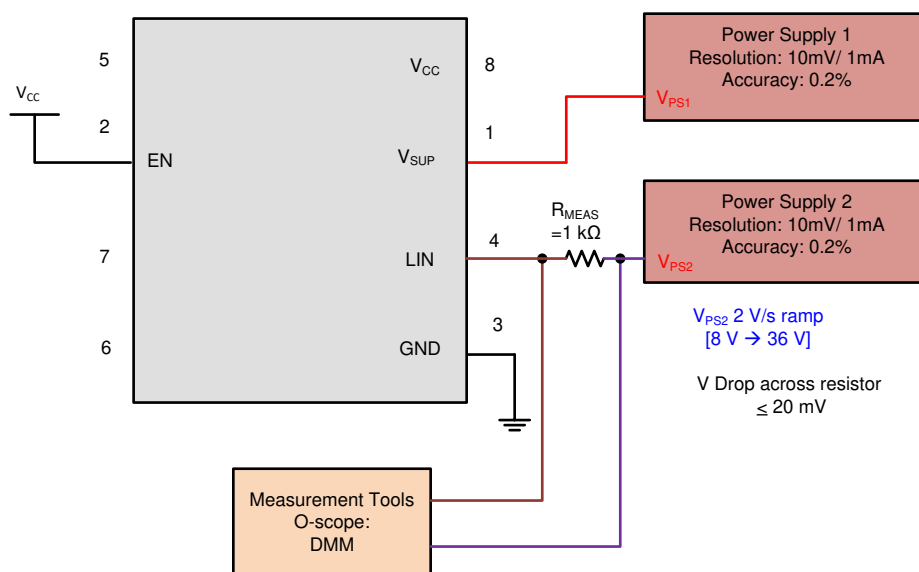
8-7. Test Circuit for I_{BUS\_PAS\_rec}
