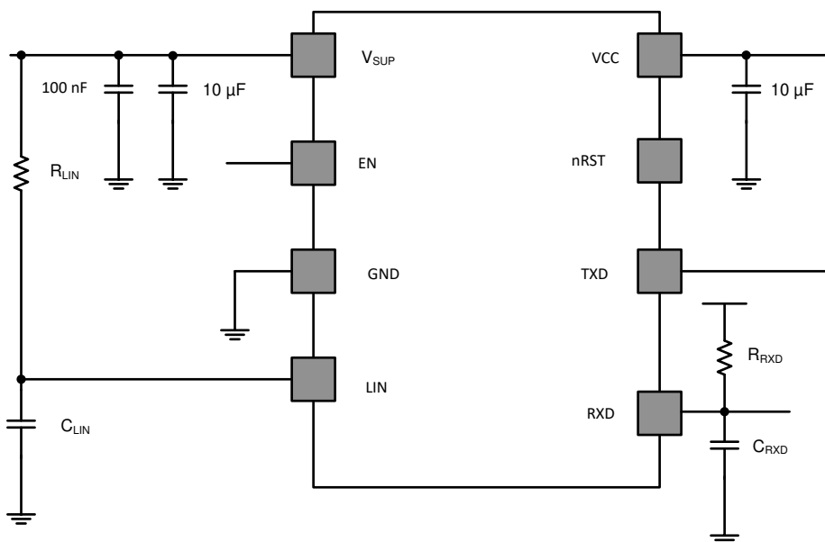
8-17. Test Circuit for AC Characteristics
