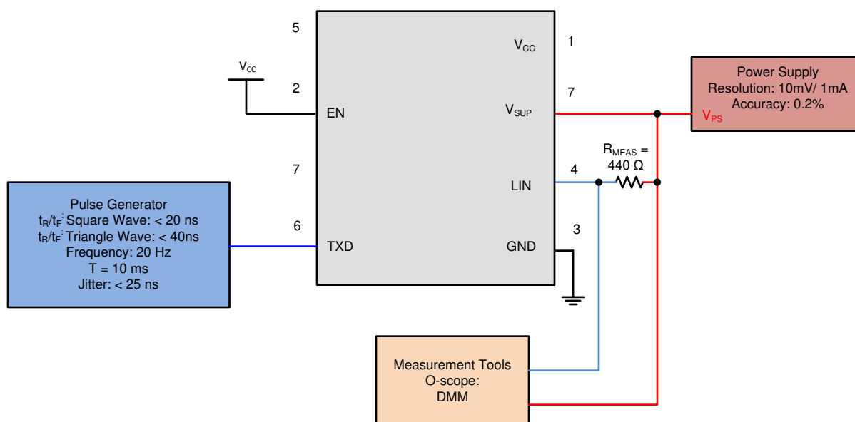
8-5. Test Circuit for I_{BUS\_LIM} at Dominant State (Driver on)
