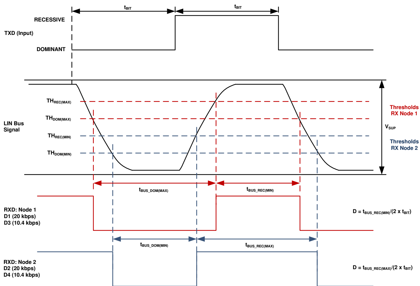
8-11. Definition of Bus Timing
