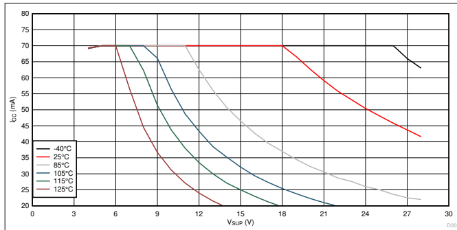
7-1. I_{CC} vs V_{SUP} vs Temperature
