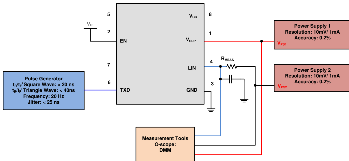
8-10. Test Circuit Slope Control and Duty Cycle
