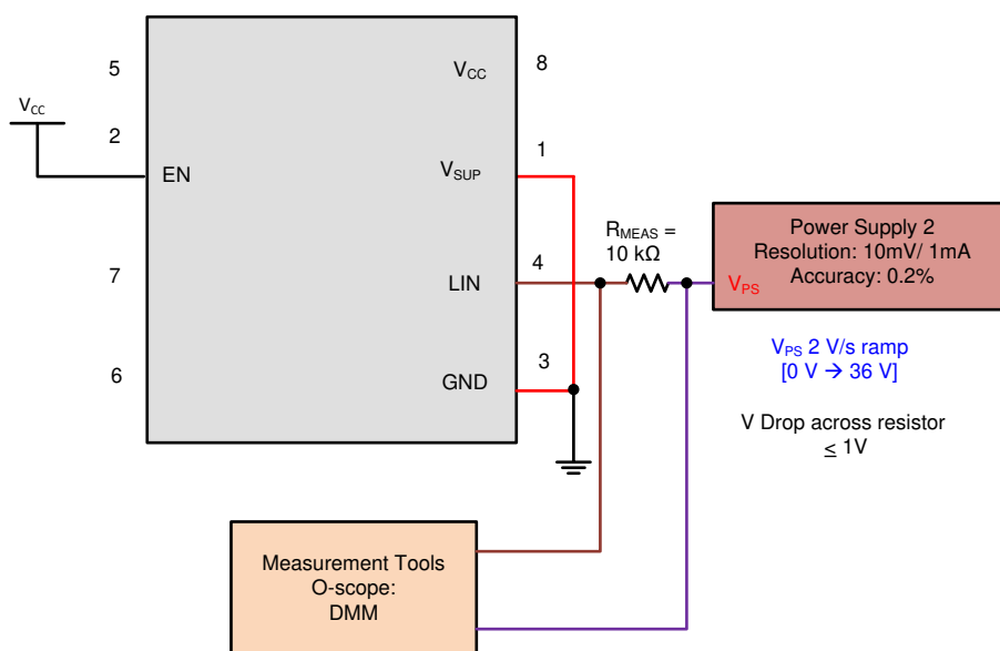
8-9. Test Circuit for I_{BUS\_NO\_BAT} Loss of Battery
