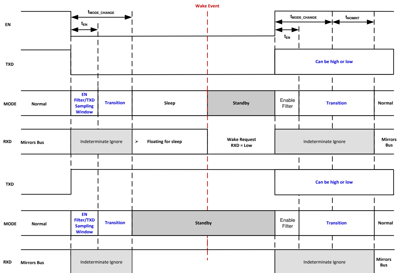
8-14. Mode Transitions
