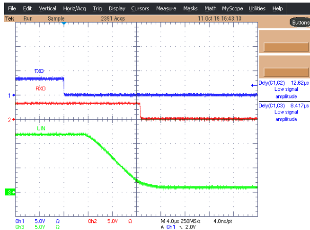
10-8. Recessive to Dominant Propagation Delay
