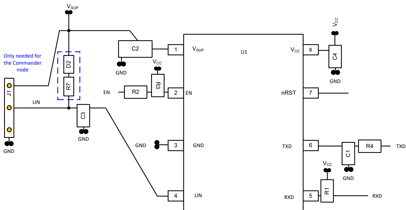
12-1. Layout Example
