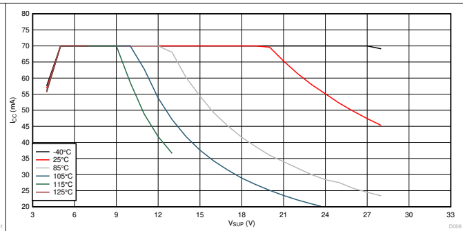
7-2. I_{CC} vs V_{SUP} vs Temperature
