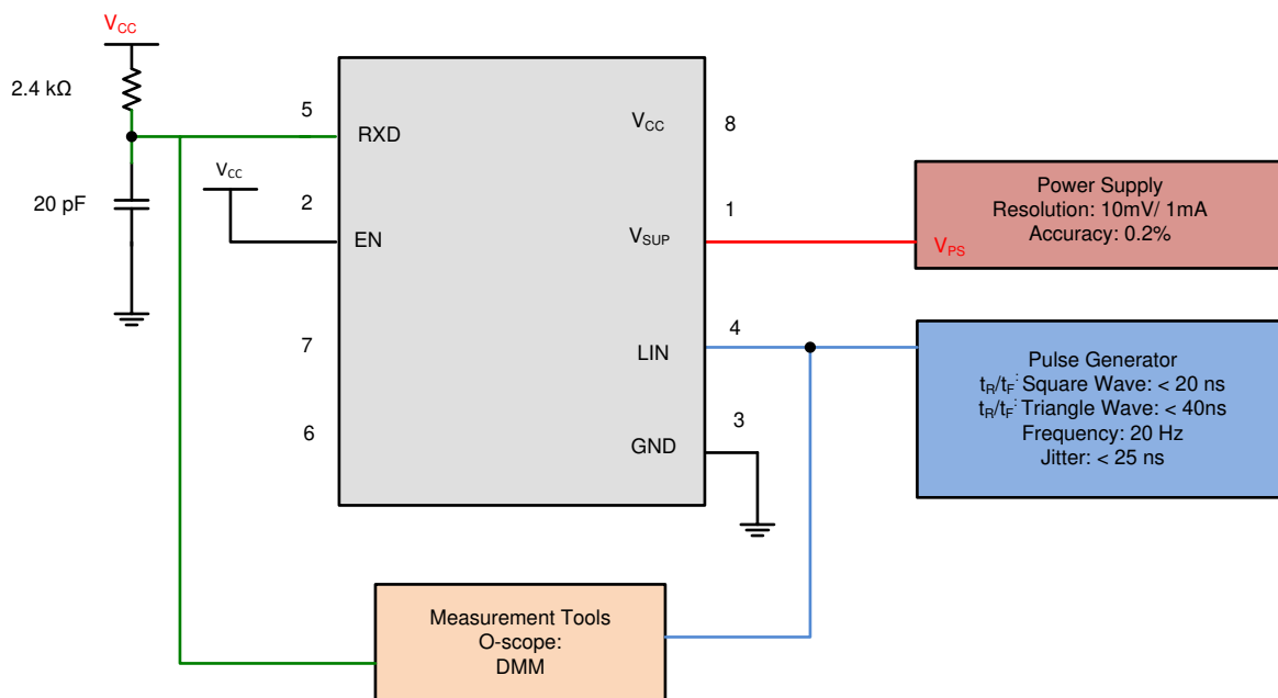
8-12. Propagation Delay Test Circuit
