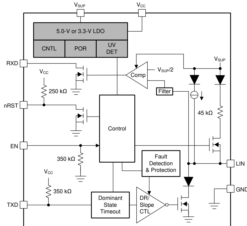
FIG 9-1. Functional Block Diagram
