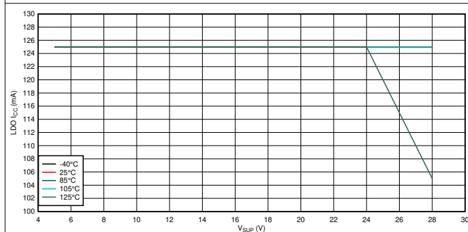
Figure 7-1. I_{CC} vs V_{SUP} vs Temperature
