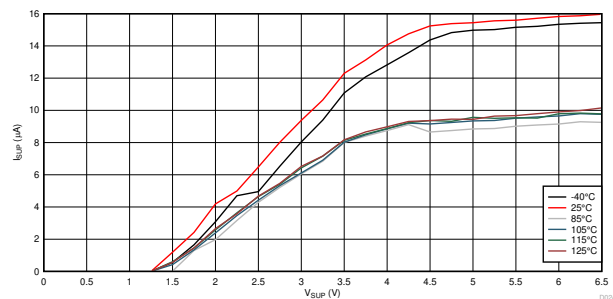
10-8. I_{SUP} vs V_{SUP} vs Temperature Ramp-down
