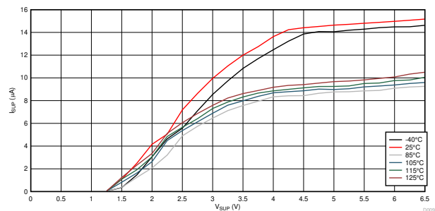
10-9. I_{SUP} vs V_{SUP} vs Temperature Ramp-down
