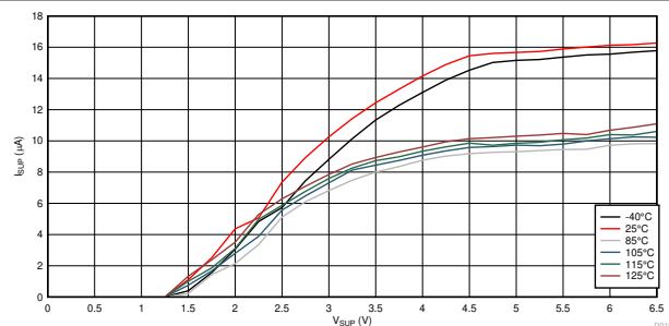
10-10. I_{SUP} vs V_{SUP} vs Temperature Ramp-down
