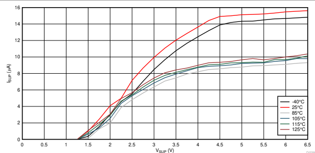
10-11. I_{SUP} vs V_{SUP} vs Temperature Ramp-down
