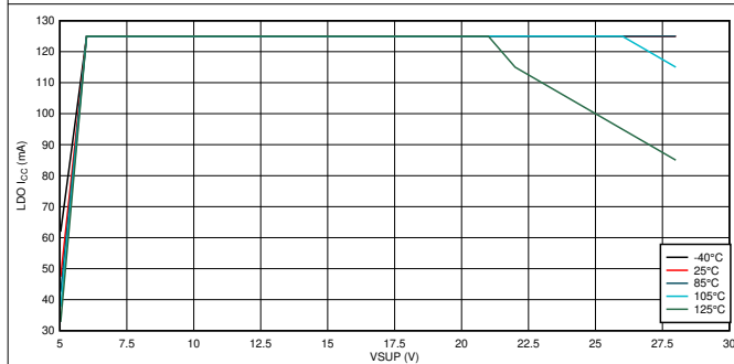
Figure 7-3. I_{CC} vs V_{SUP} vs Temperature
