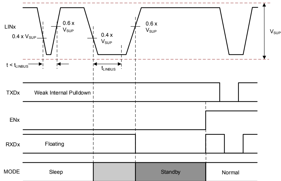
図 8-16. Wake-Up Through LIN
