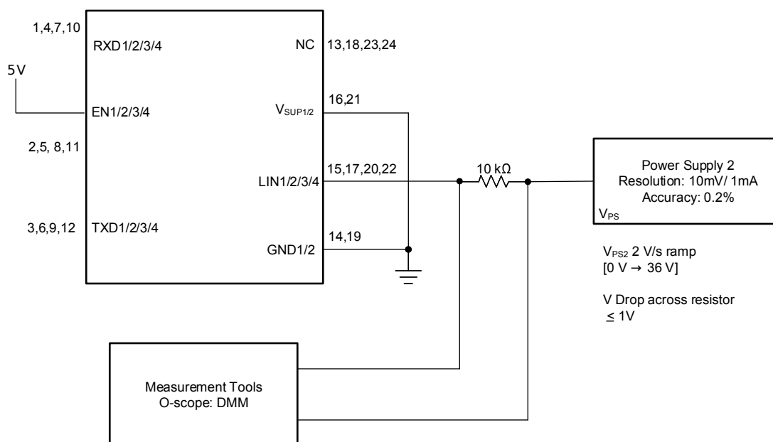
8-9. Test Circuit for I_{BUS \text{ NO BAT}} Loss of Battery
