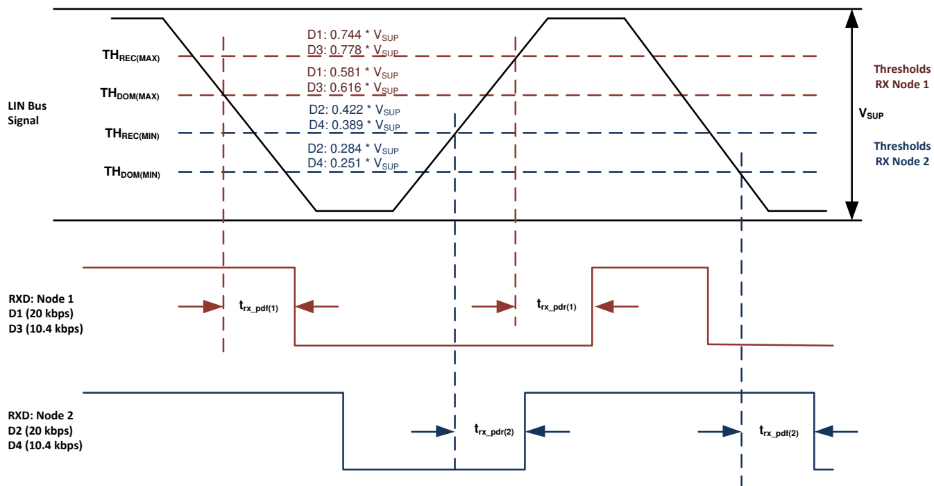
8-13. Propagation Delay
