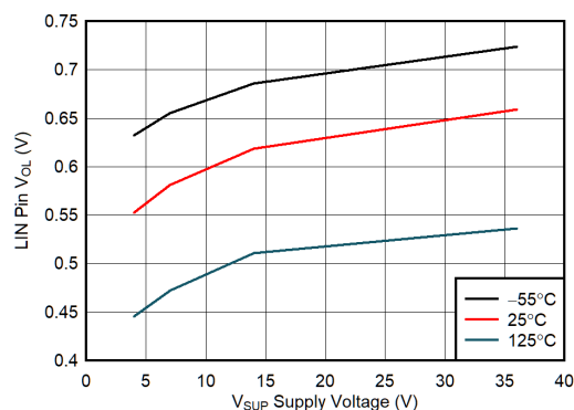
7-2. V_{OL} vs V_{SUP} and Temperature
