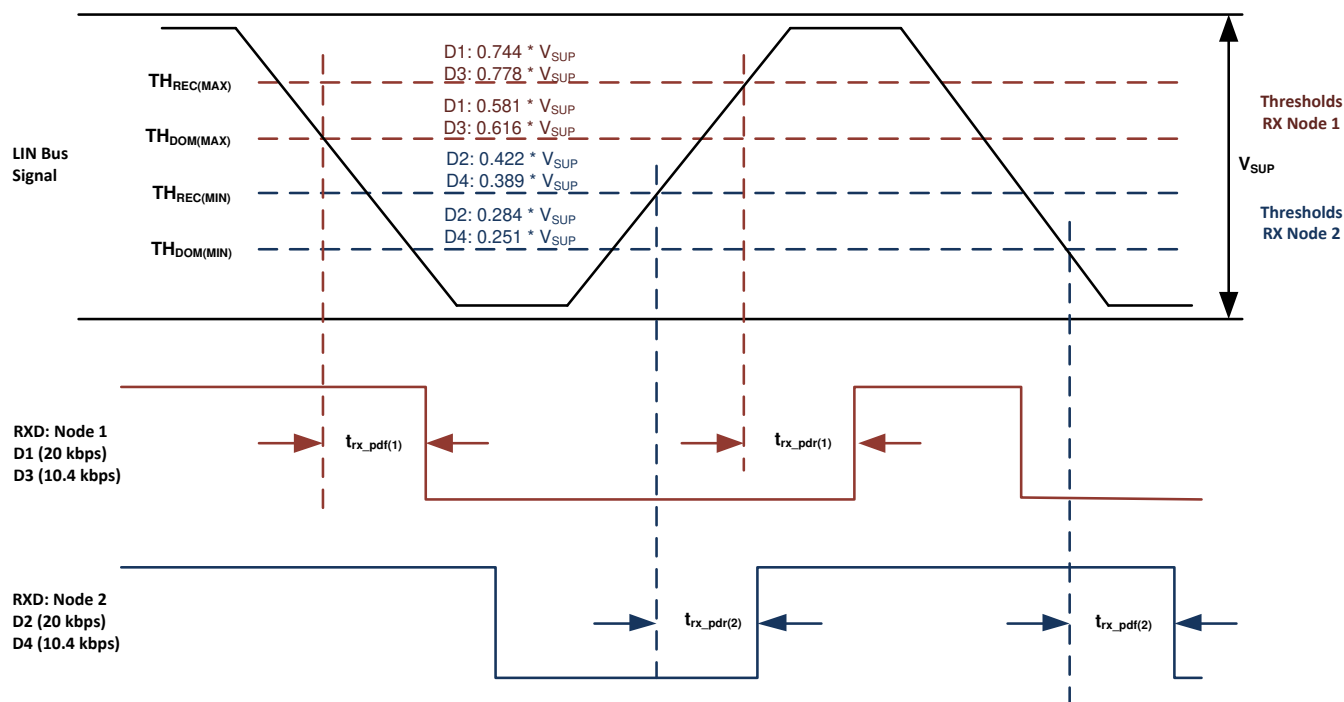
8-13. Propagation Delay
