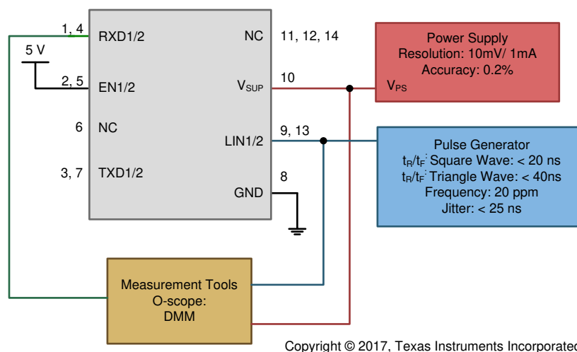
FIG 7-1. Test System: Operating Voltage Range with RX and TX Access: Parameters 9, 10
