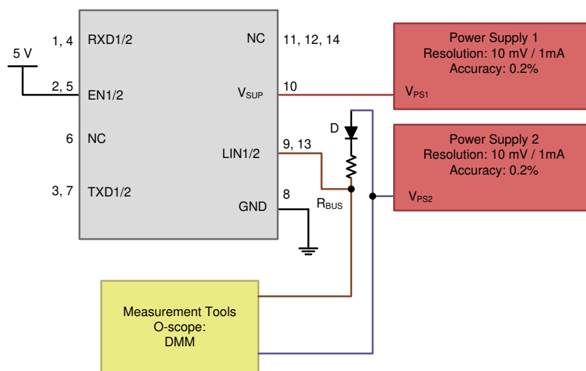
7-4. LIN Receiver Test with RX access Parameters 17, 18, 19, 20
