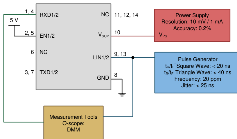
7-4. LIN Receiver Test with RX access Parameters 17, 18, 19, 20
