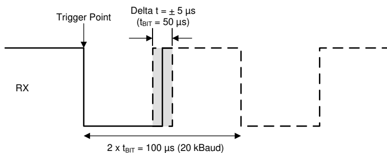
FIG 7-1. Test System: Operating Voltage Range with RX and TX Access: Parameters 9, 10
