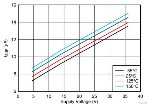
Figure 7-7. Sleep mode I_{SUP} vs V_{SUP} and Temperature
