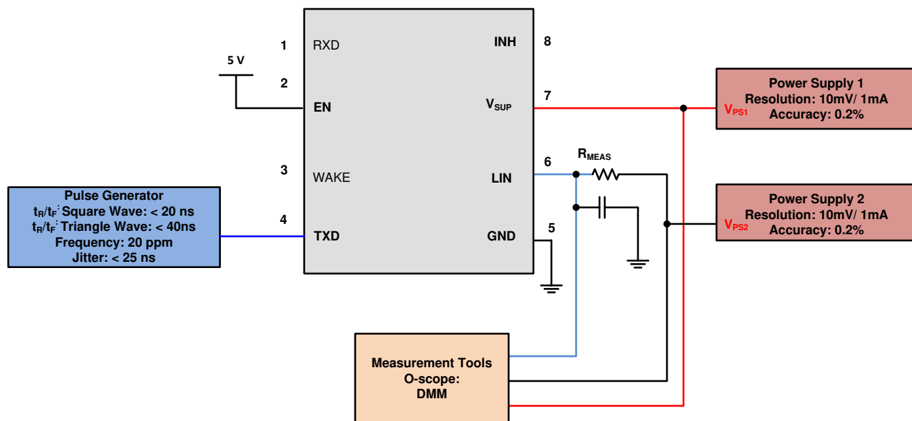
8-8. Test Circuit Slope Control and Duty Cycle Param 27, 28, 29, 30
