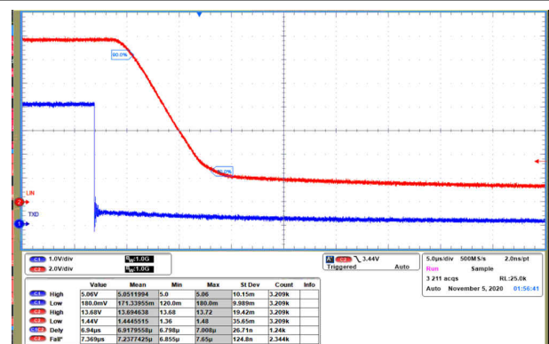
Figure 10-3. Recessive to Dominant Propagation Delay
