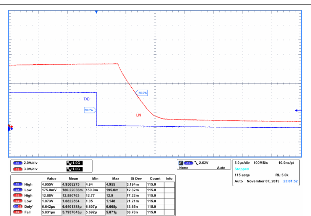
10-3. Recessive to Dominant Propagation Delay
