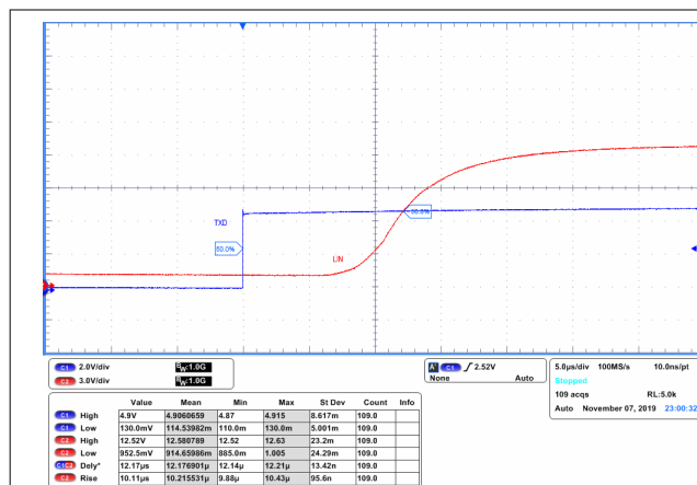
10-2. Dominant To Recessive Propagation Delay
