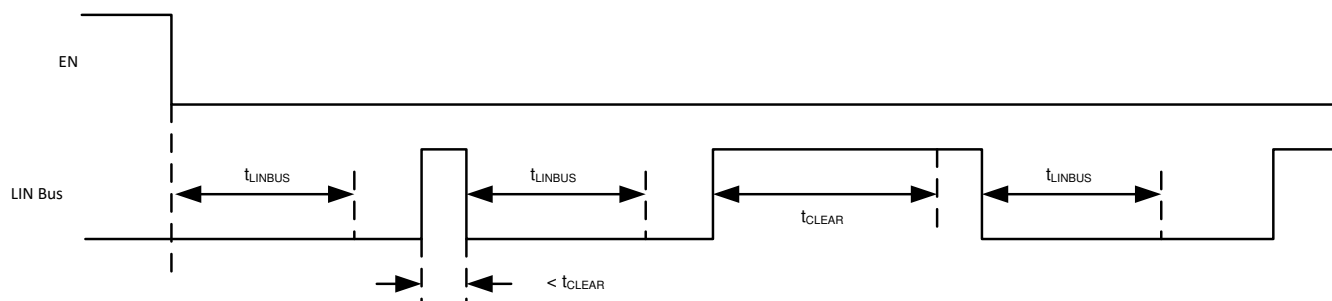
☒ 9-2. No Bus Fault: Entering Sleep Mode with Bus Recessive Condition and Wake-up
