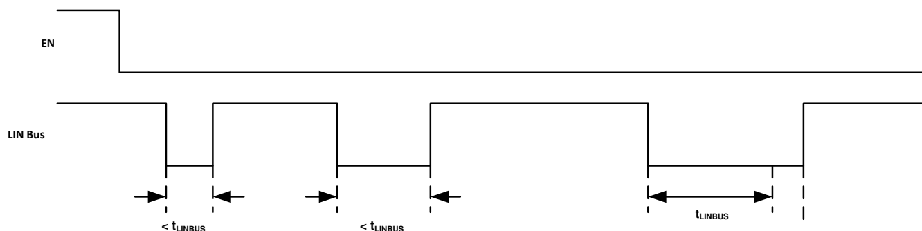
☒ 9-2. No Bus Fault: Entering Sleep Mode with Bus Recessive Condition and Wake-up
