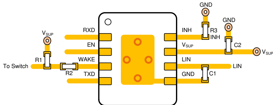
Figure 10-4. Layout Example
