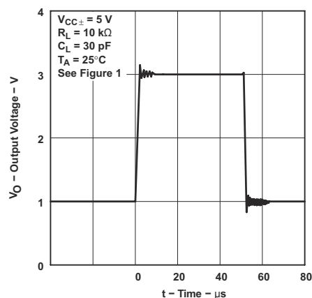
Figure 5-50. TLE2024xM Voltage-Follower Large-Scale Pulse Response
