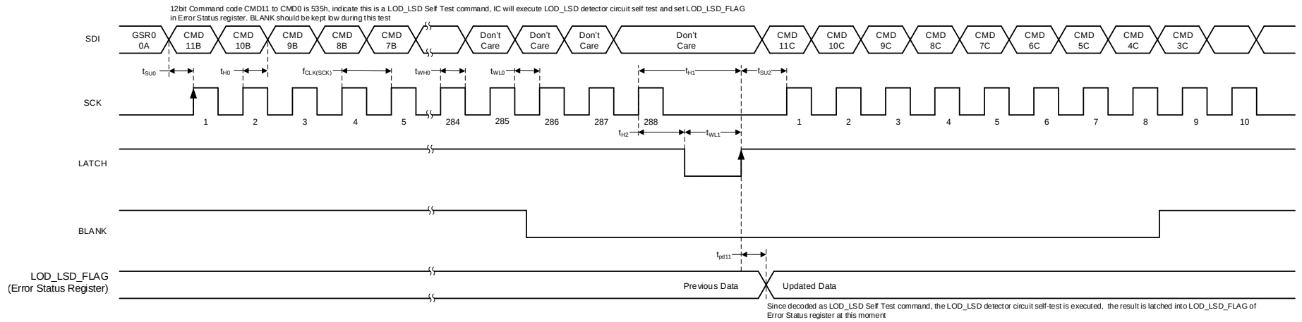
图 7. LOD_LSD Self-Test
