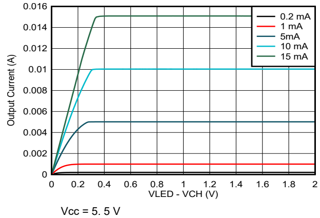
7-3. Channel Current vs (VLED-Vchannel) Voltage
