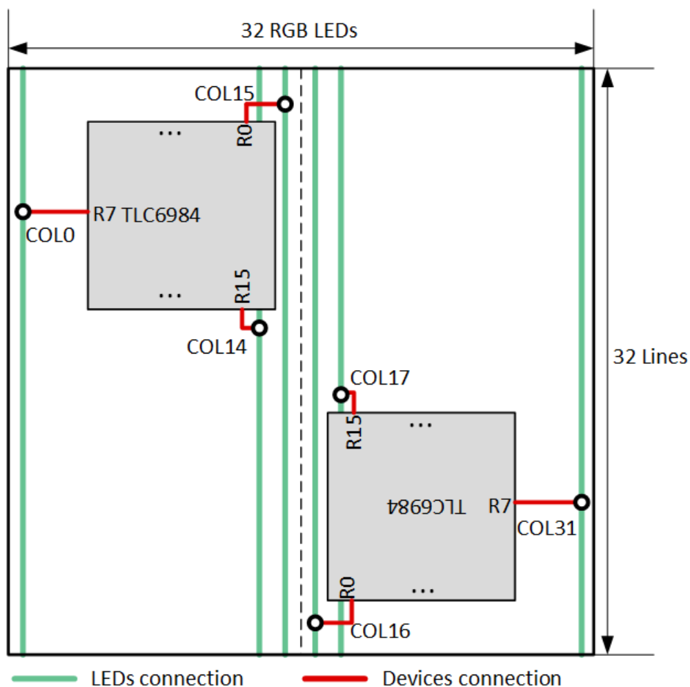
FIG 11-3. Channel Routing Suggestion With Shortest Wire
