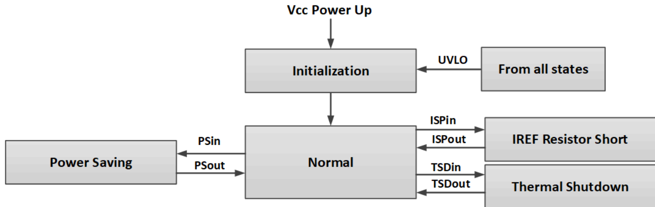
FIG 8-16. Functional Modes
