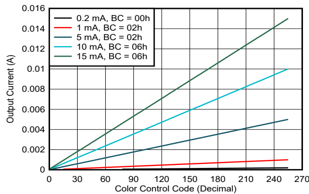
7-6. Color Control Code vs Output Current
