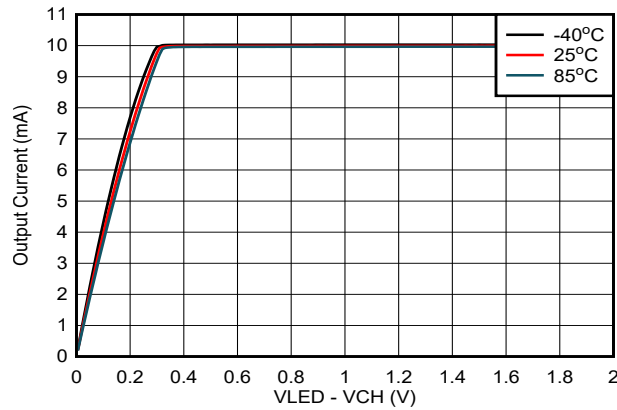
7-4. Channel Current vs (VLED-Vchannel) Voltage
