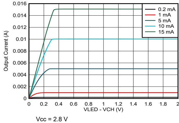
7-2. Channel Current vs (VLED-Vchannel) Voltage
