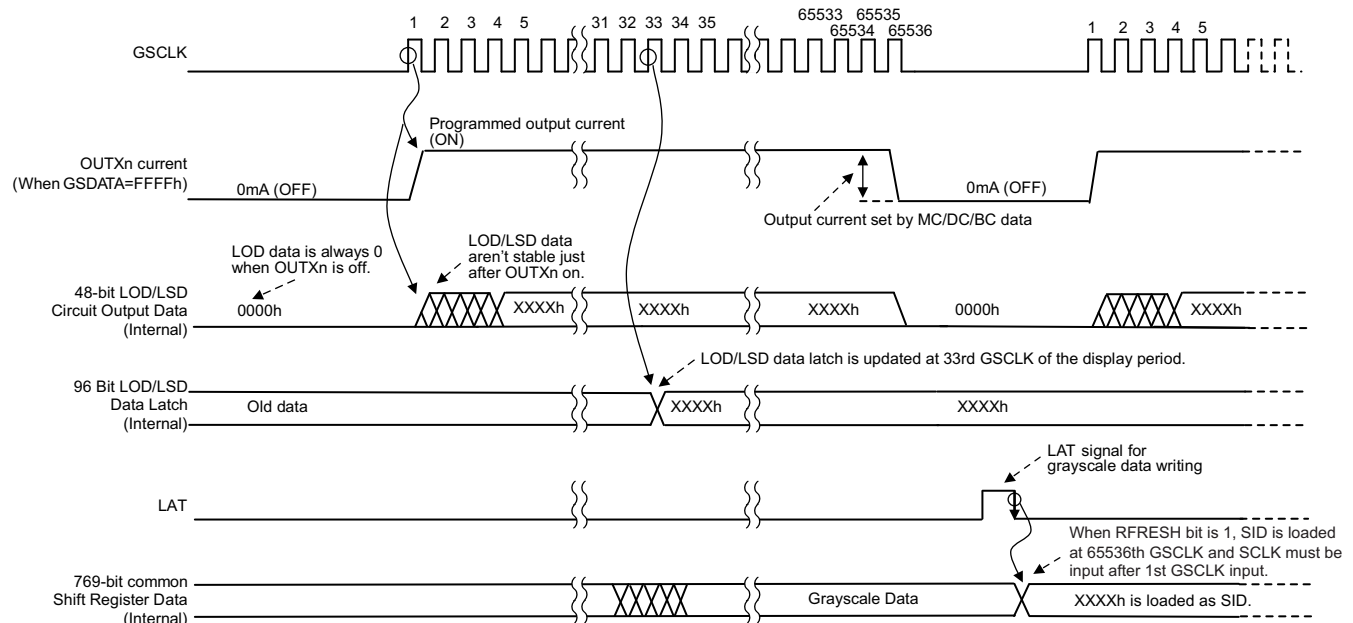
Figure 26. LOD and LSD Read and Load Timing Diagram
