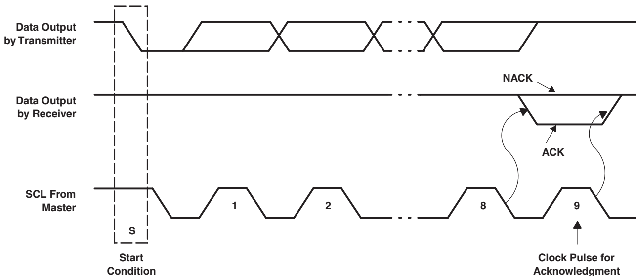
Figure 12. Acknowledge/Not Acknowledge on I²C Bus
