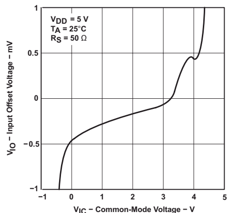
Figure 6-5. Input Offset Voltage vs Common-Mode Voltage
