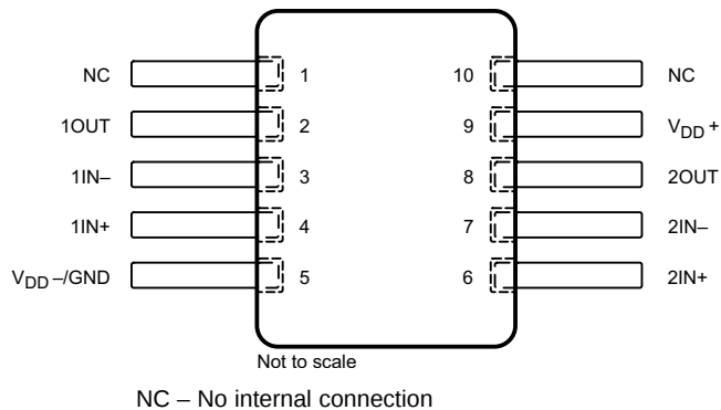
U Package 10-Pin CFP Top View
