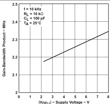
FIG 6-55. Gain-Bandwidth Product vs Supply Voltage
