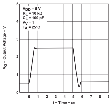
6-44. Voltage-Follower Large-Signal Pulse Response
