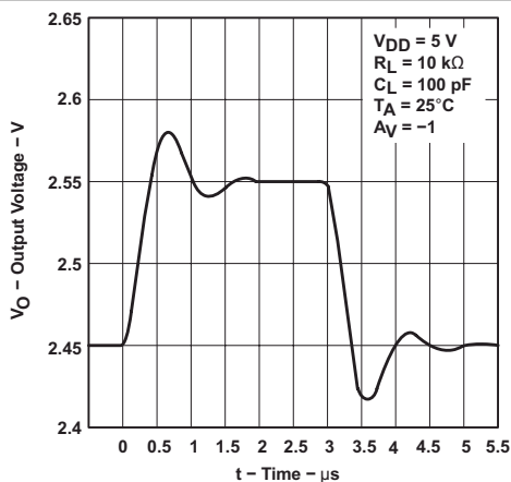
6-46. Inverting Small-Signal Pulse Response
