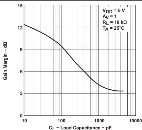
FIG 6-58. Gain Margin vs Load Capacitance
