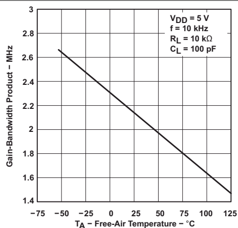
FIG 6-56. Gain-Bandwidth Product vs Free-Air Temperature
