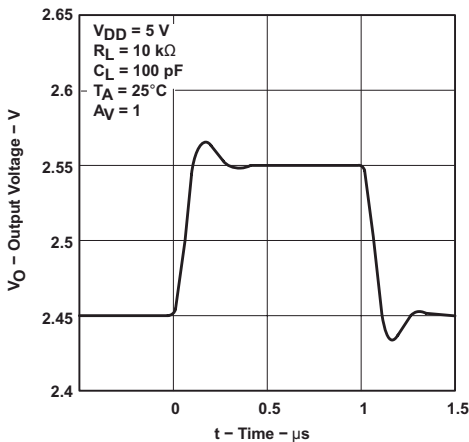
6-48. Voltage-Follower Small-Signal Pulse Response
