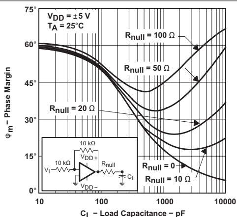
FIG 6-57. Phase Margin vs Load Capacitance
