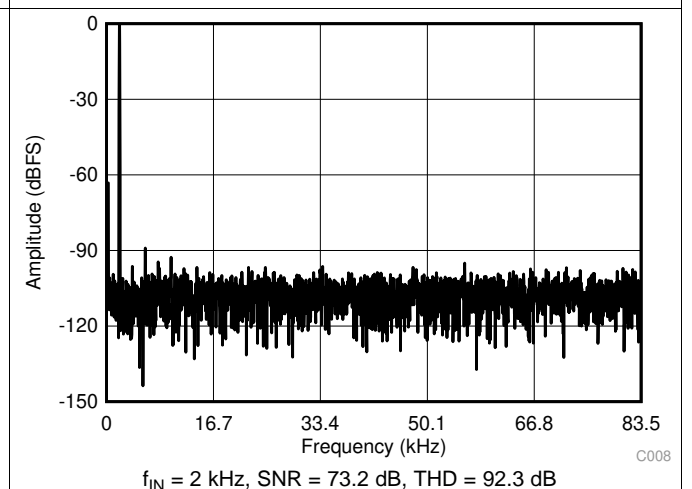
Figure 13. Typical FFT
